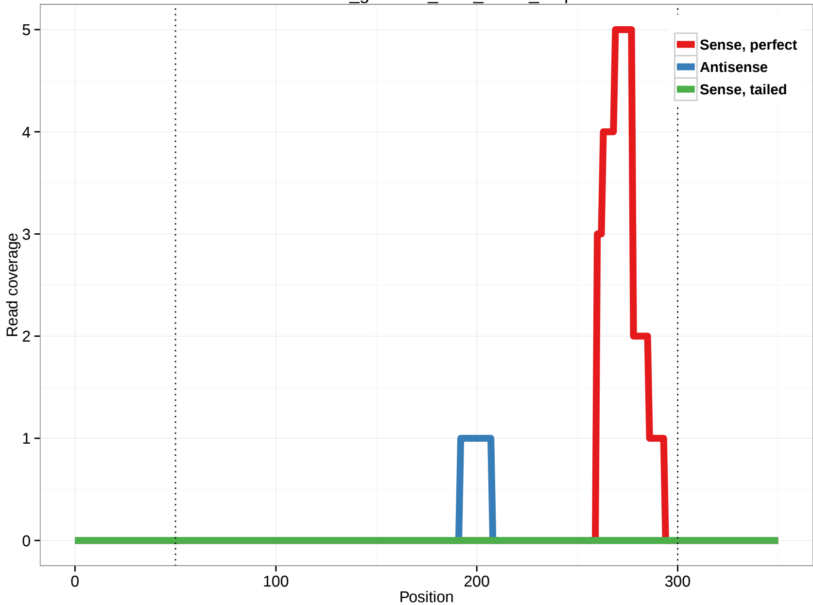
rheMac3_genscan_chr3_291.2_4.5p
