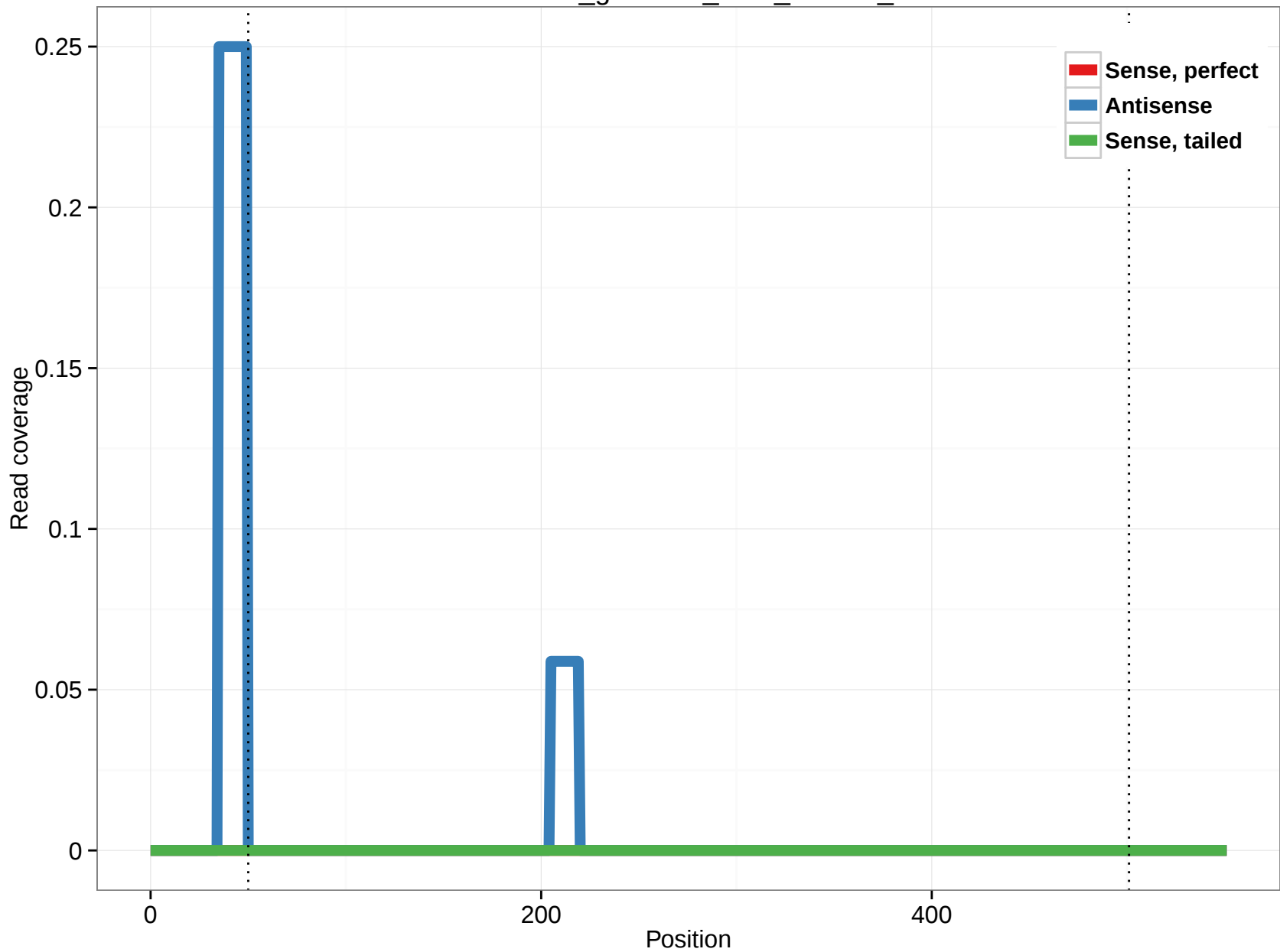
rheMac3_genscan_chr3_288.36_2
