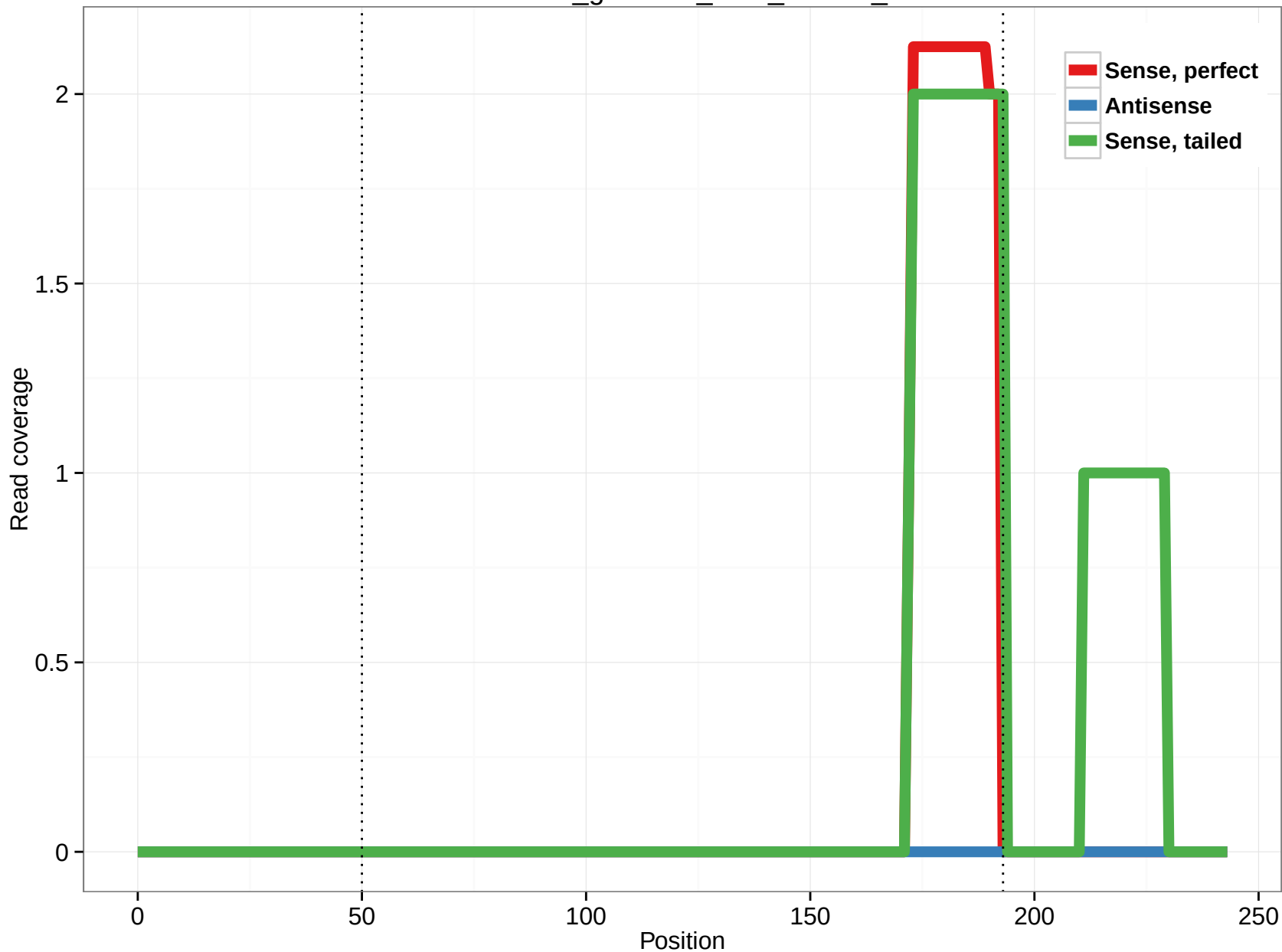
rheMac3_genscan_chr3_288.36_1
