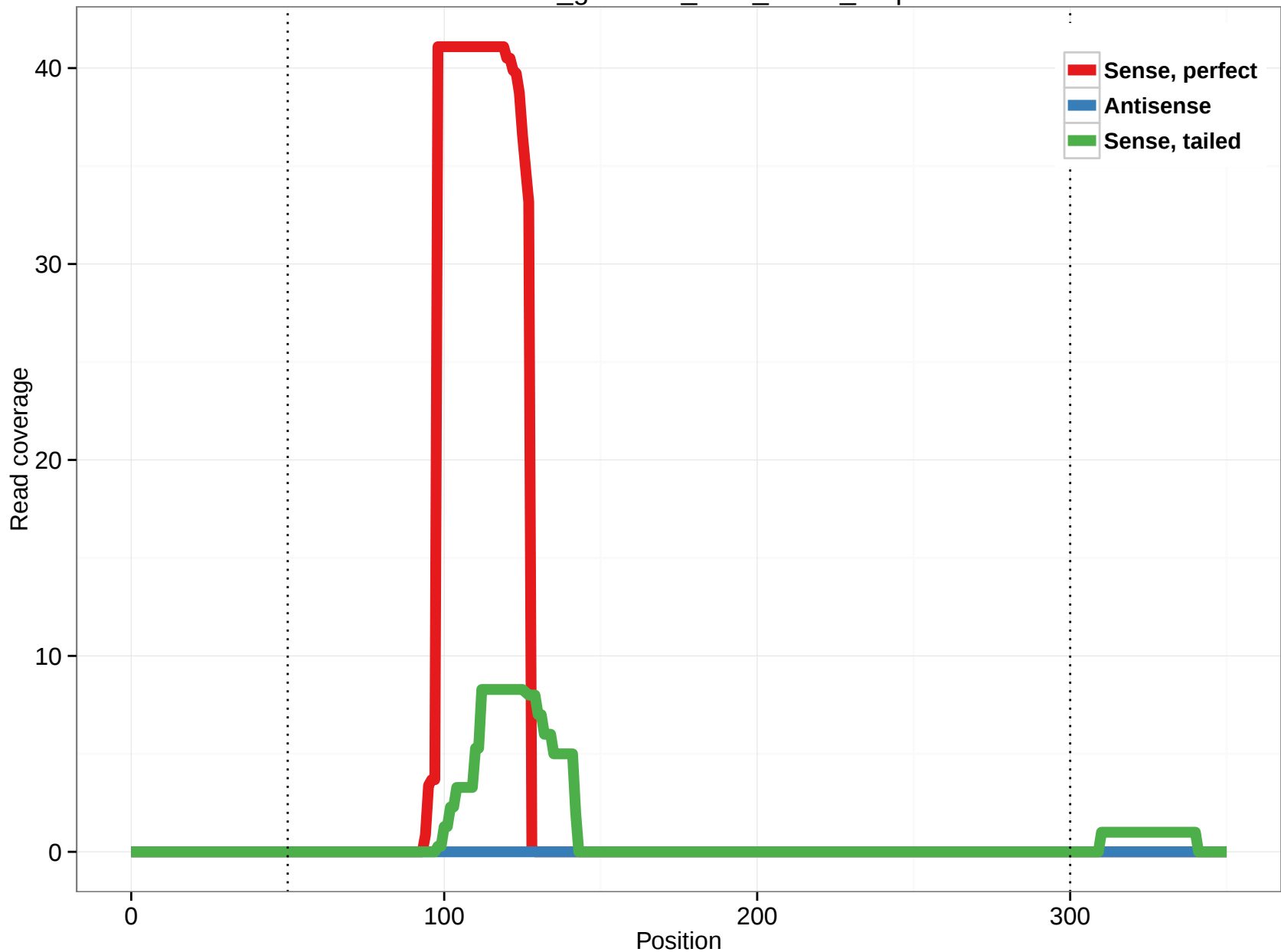
rheMac3_genscan_chr3_283.8_1.5p
