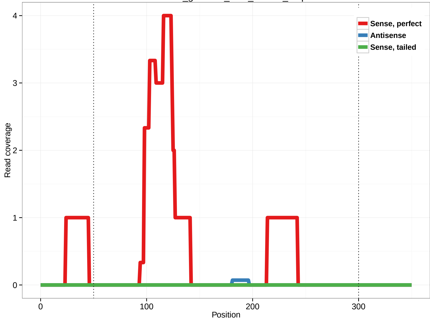
rheMac3_genscan_chr3_283.25_2.5p
