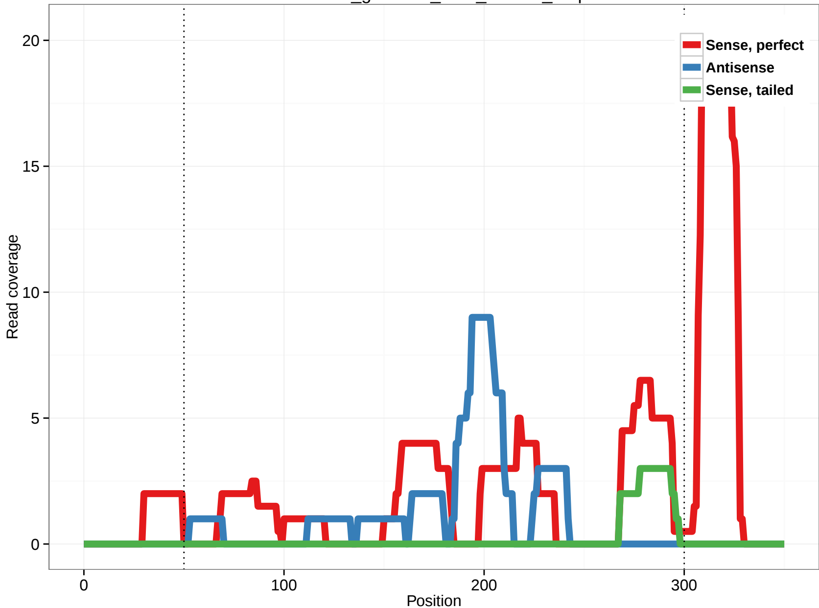
rheMac3_genscan_chr3_283.25_0.3p
