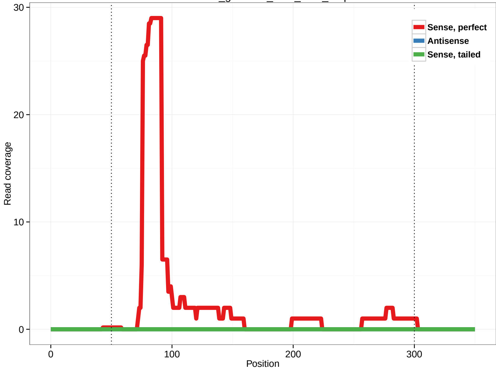
rheMac3_genscan_chr3_28.5_4.5p
