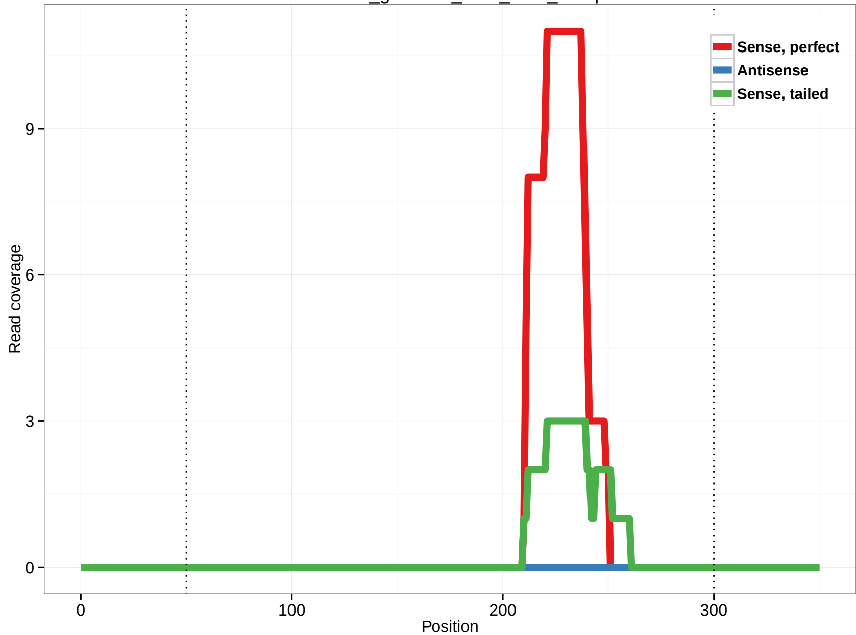
rheMac3_genscan_chr3_28.5_12.3p
