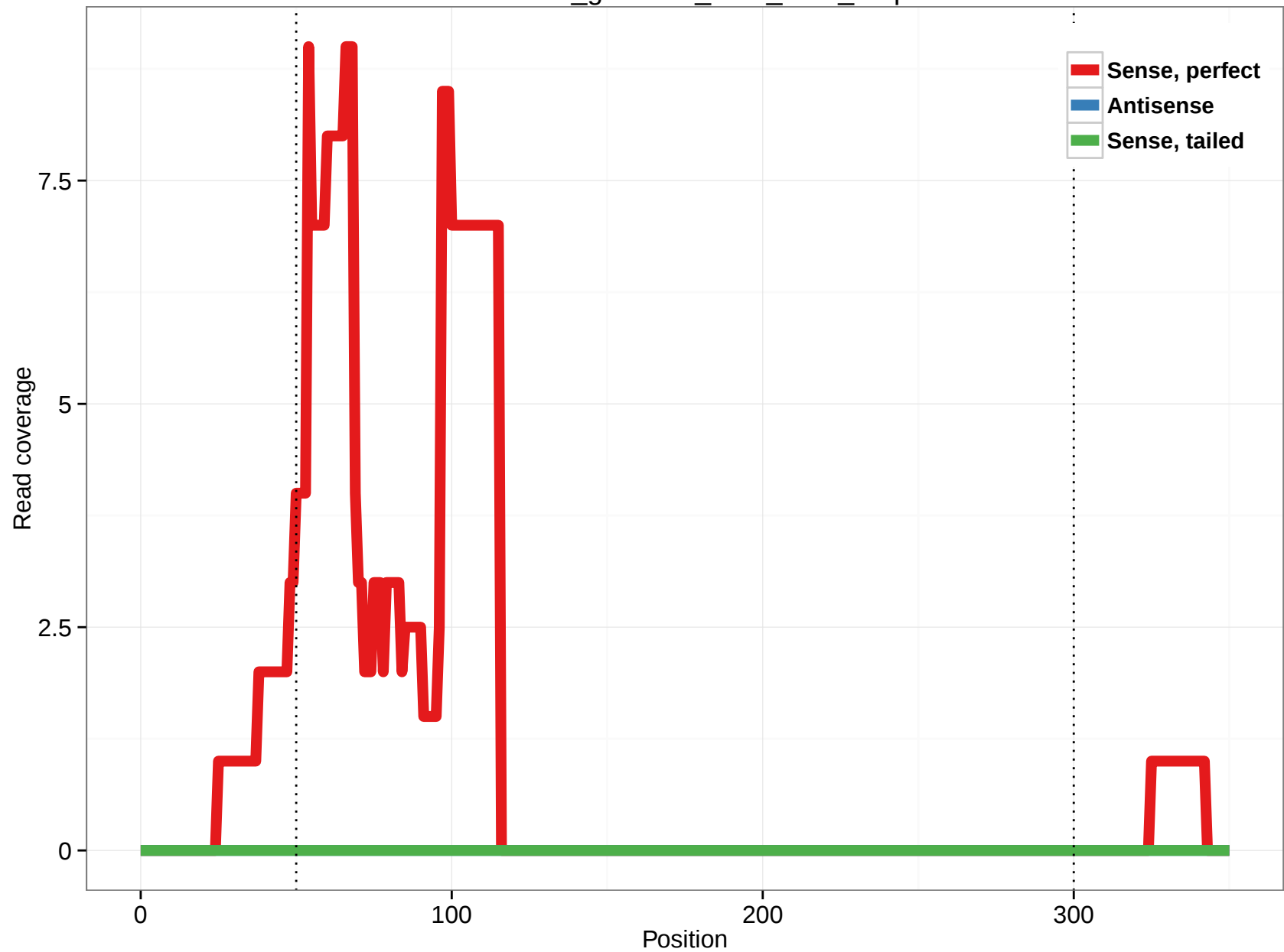
rheMac3_genscan_chr3_28.2_2.5p
