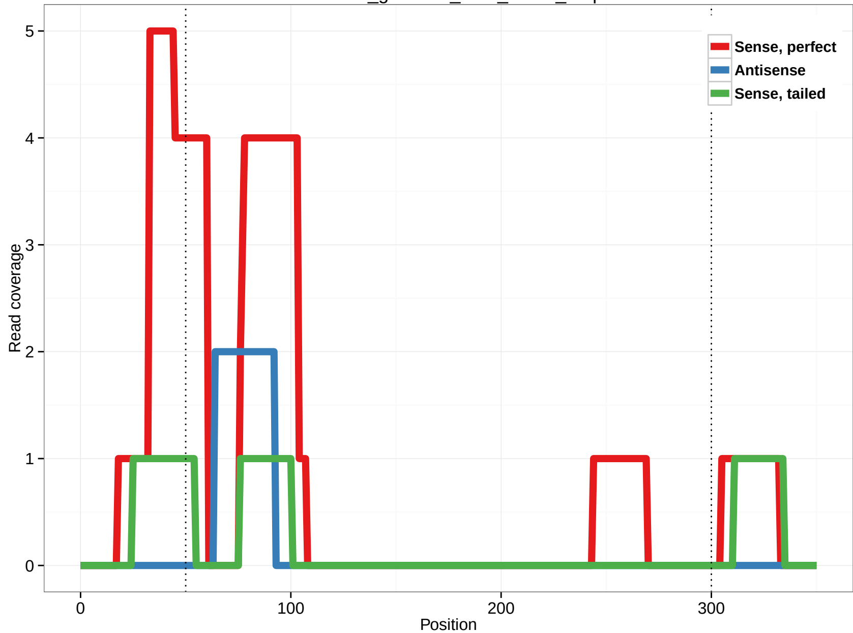
rheMac3_genscan_chr3_278.4_3.5p
