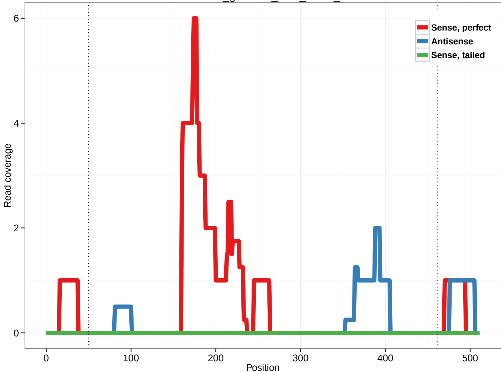
rheMac3_genscan_chr3_272.8_3
