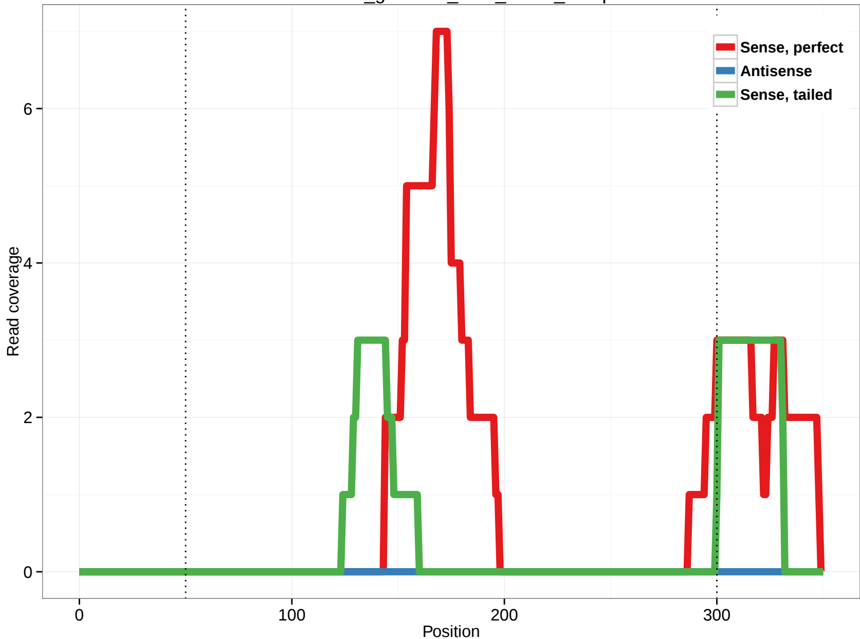
rheMac3_genscan_chr3_270.5_14.5p
