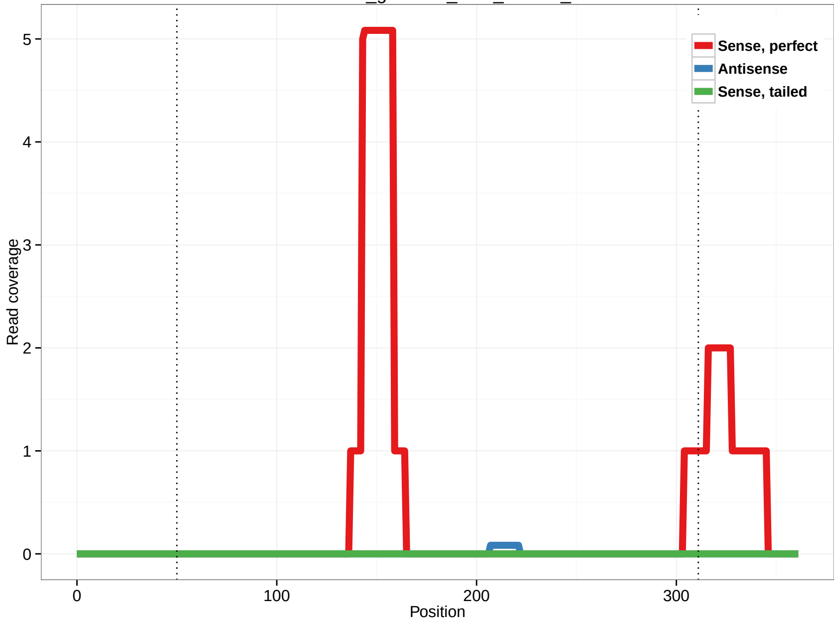
rheMac3_genscan_chr3_268.11_9
