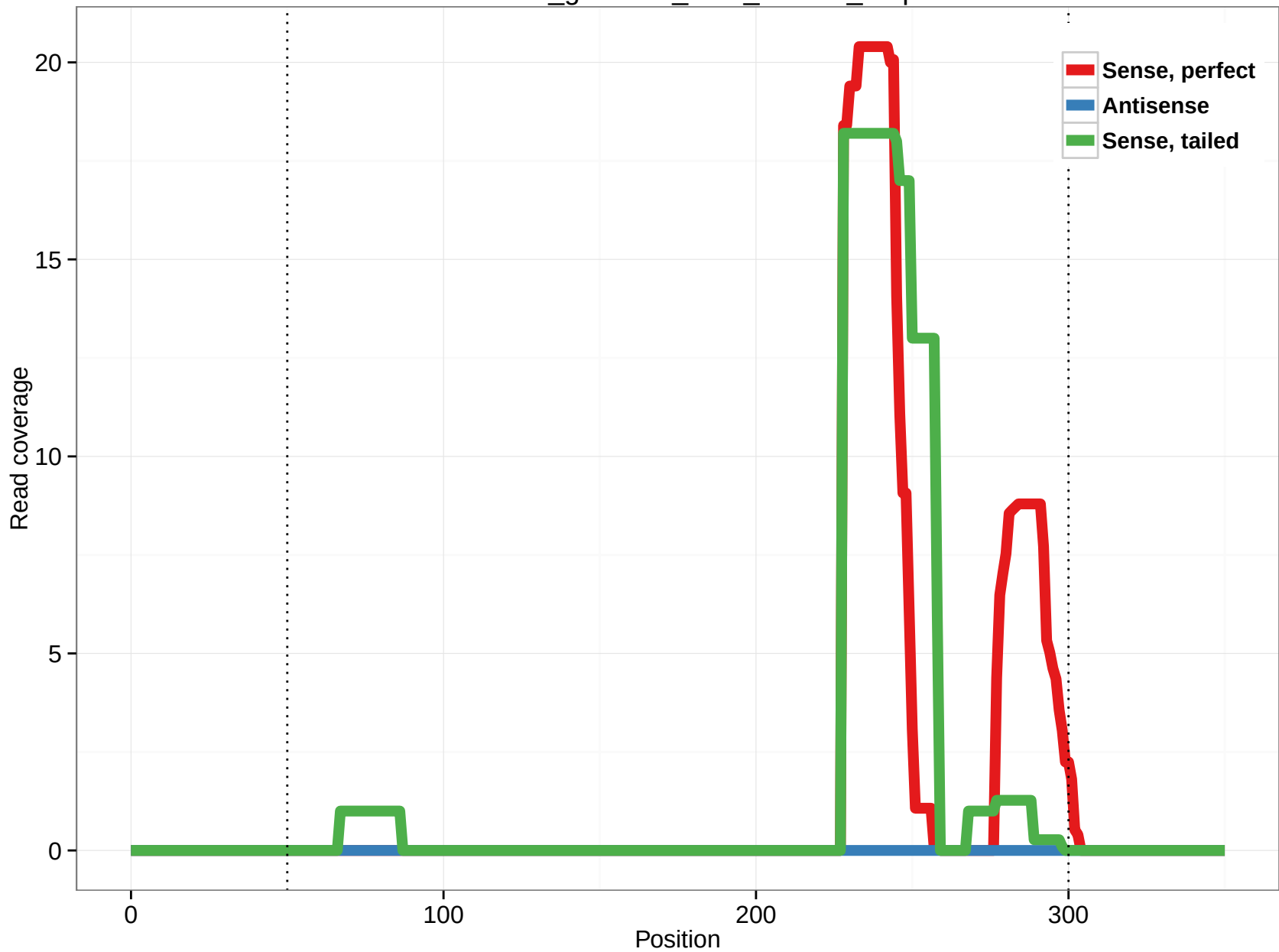
rheMac3_genscan_chr3_268.10_8.5p
