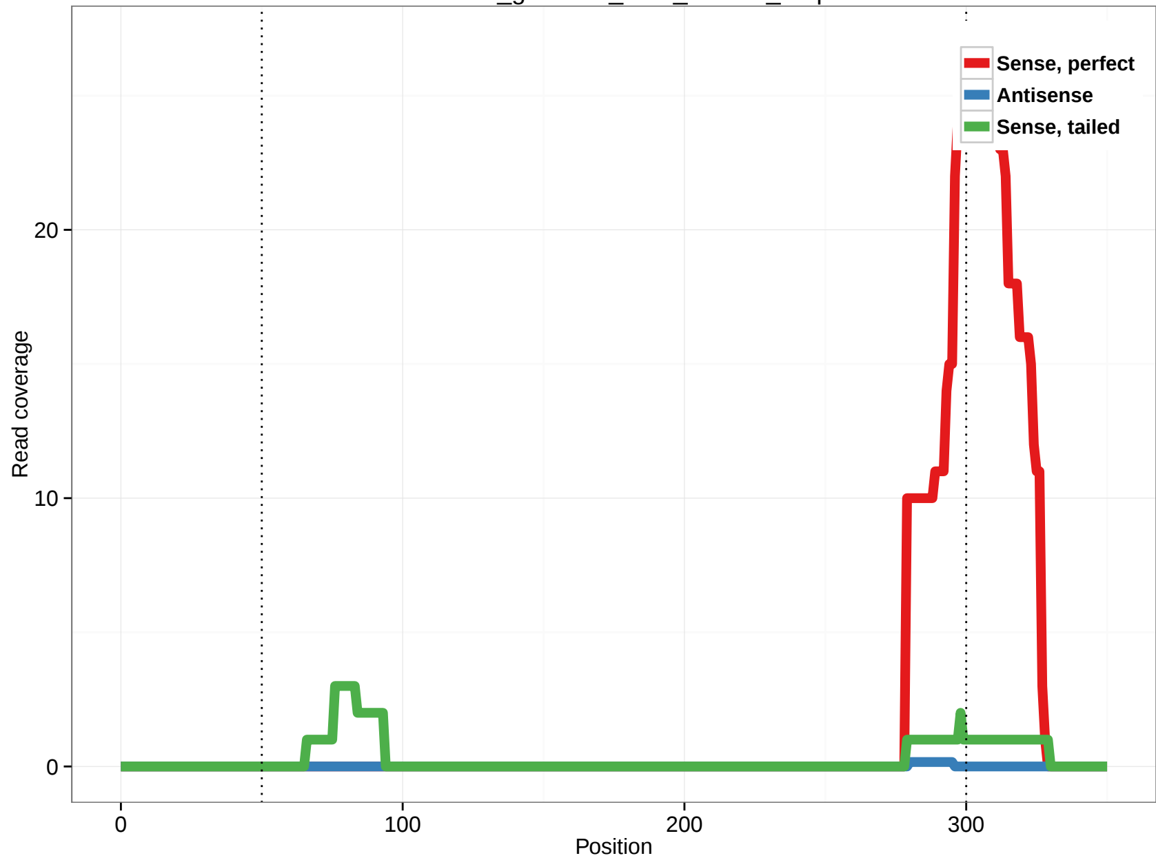
rheMac3_genscan_chr3_267.57_0.3p
