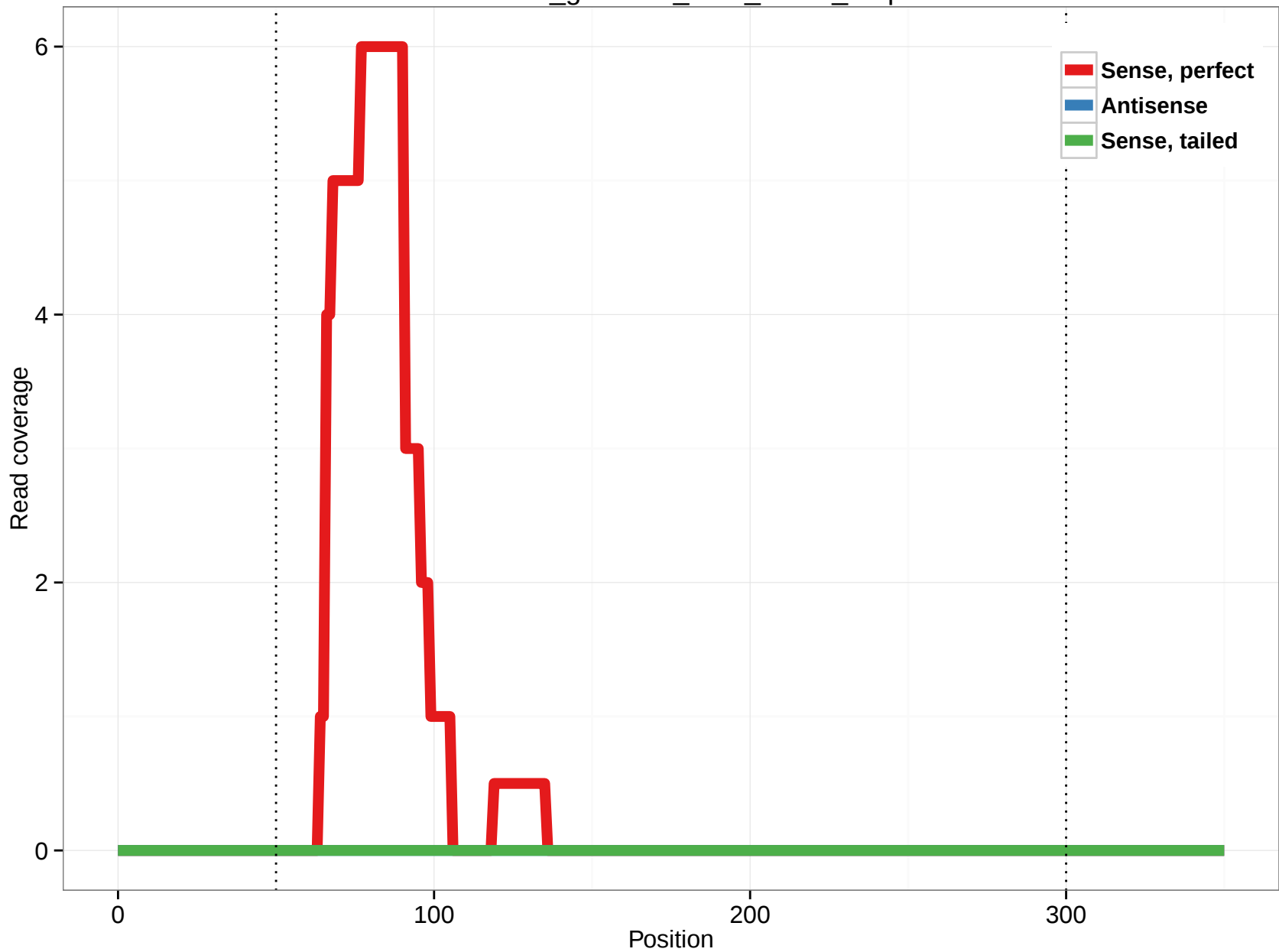
rheMac3_genscan_chr3_263.6_6.5p
