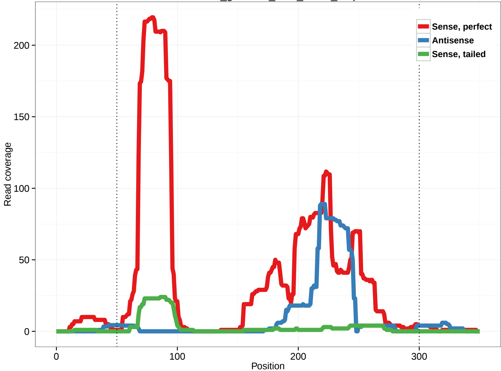
rheMac3_genscan_chr3_263.6_1.5p
