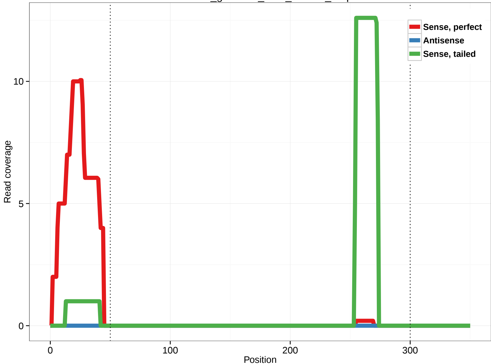
rheMac3_genscan_chr3_247.83_2.5p
