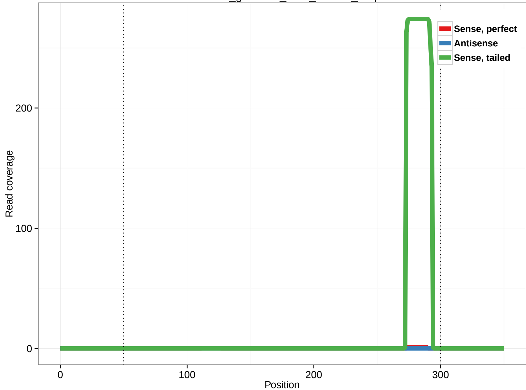
rheMac3_genscan_chr3_247.50_7.5p
