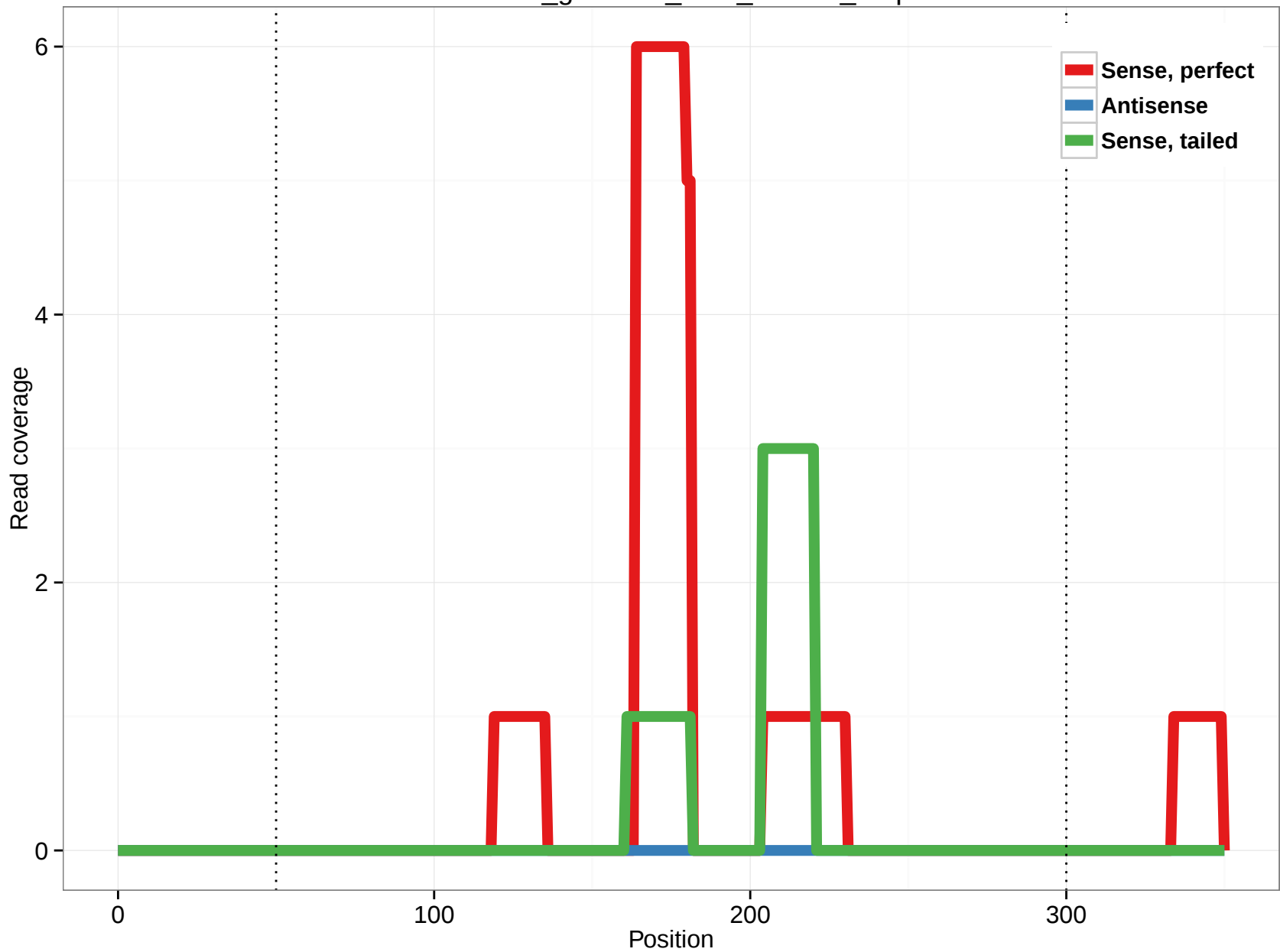
rheMac3_genscan_chr3_247.19_0.3p
