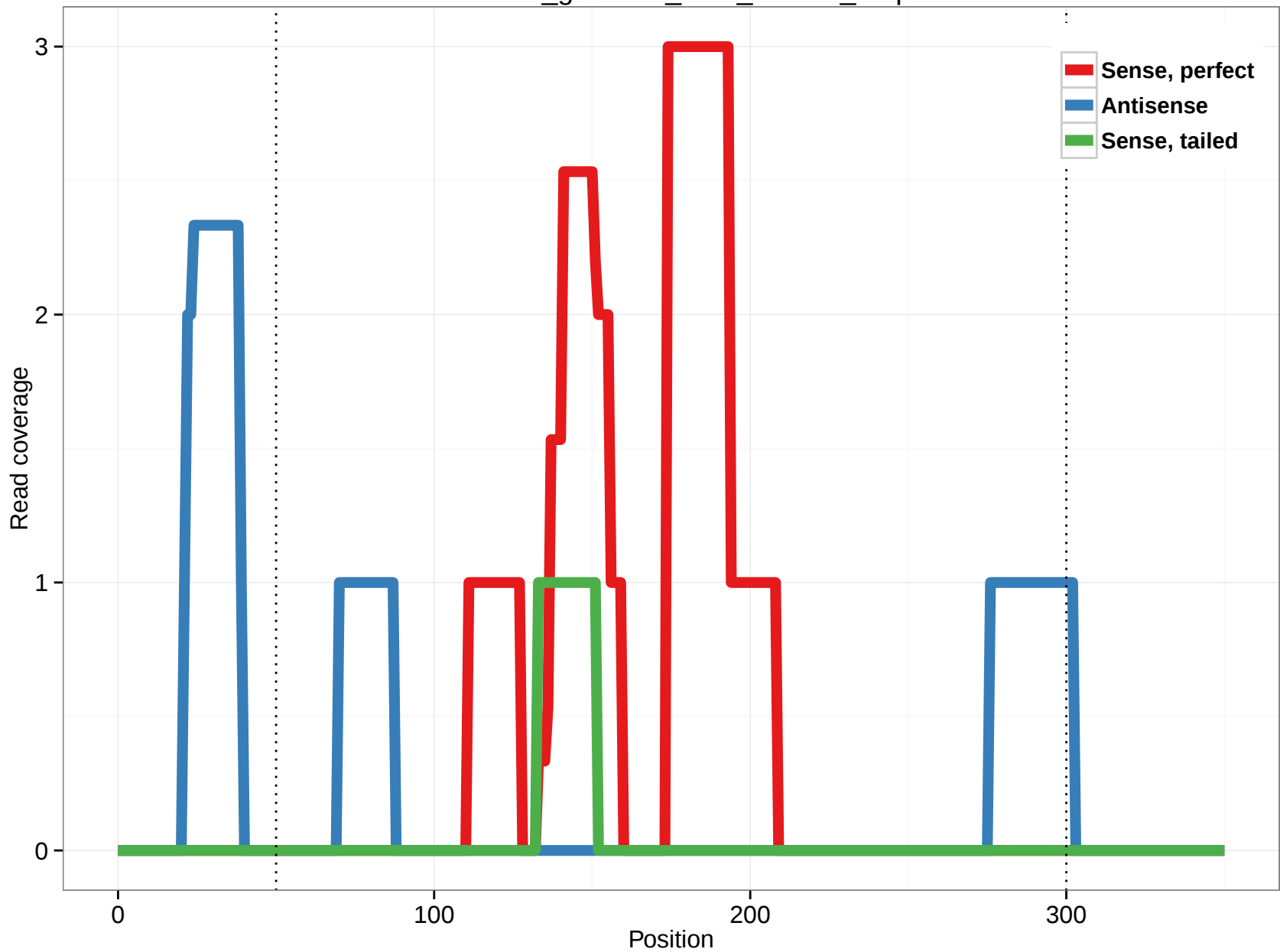
rheMac3_genscan_chr3_247.14_1.5p
