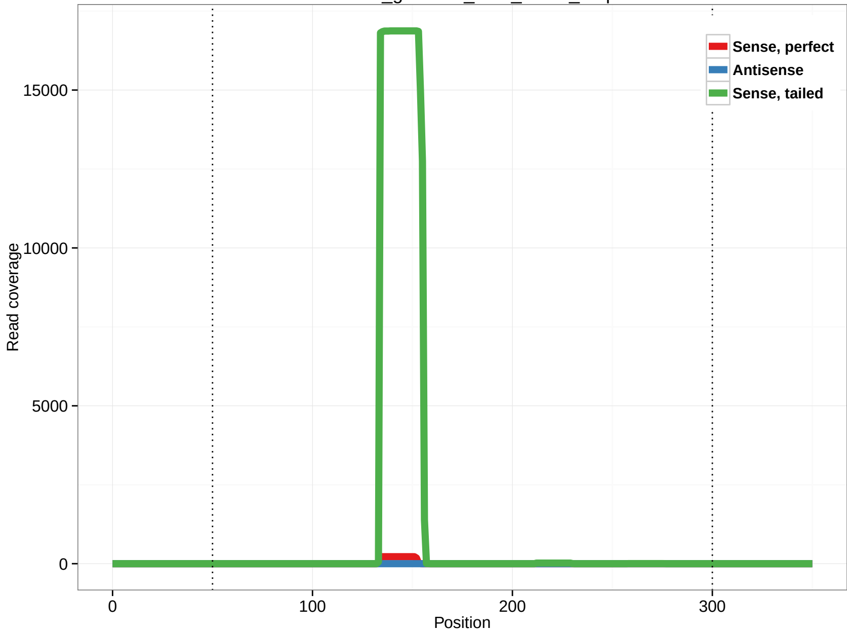
rheMac3_genscan_chr3_245.3_8.5p
