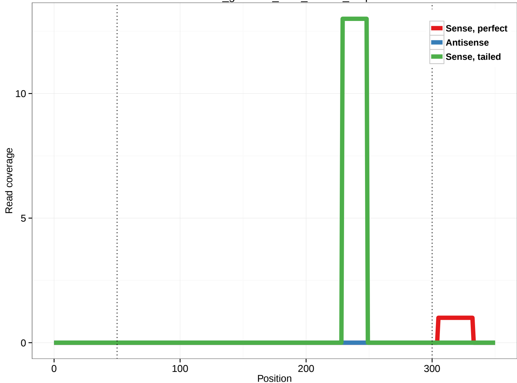
rheMac3_genscan_chr3_238.12_6.3p
