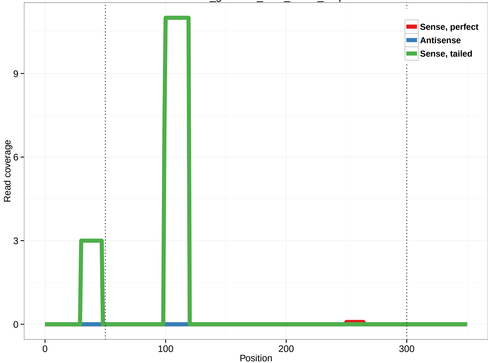
rheMac3_genscan_chr3_223.3_0.5p
