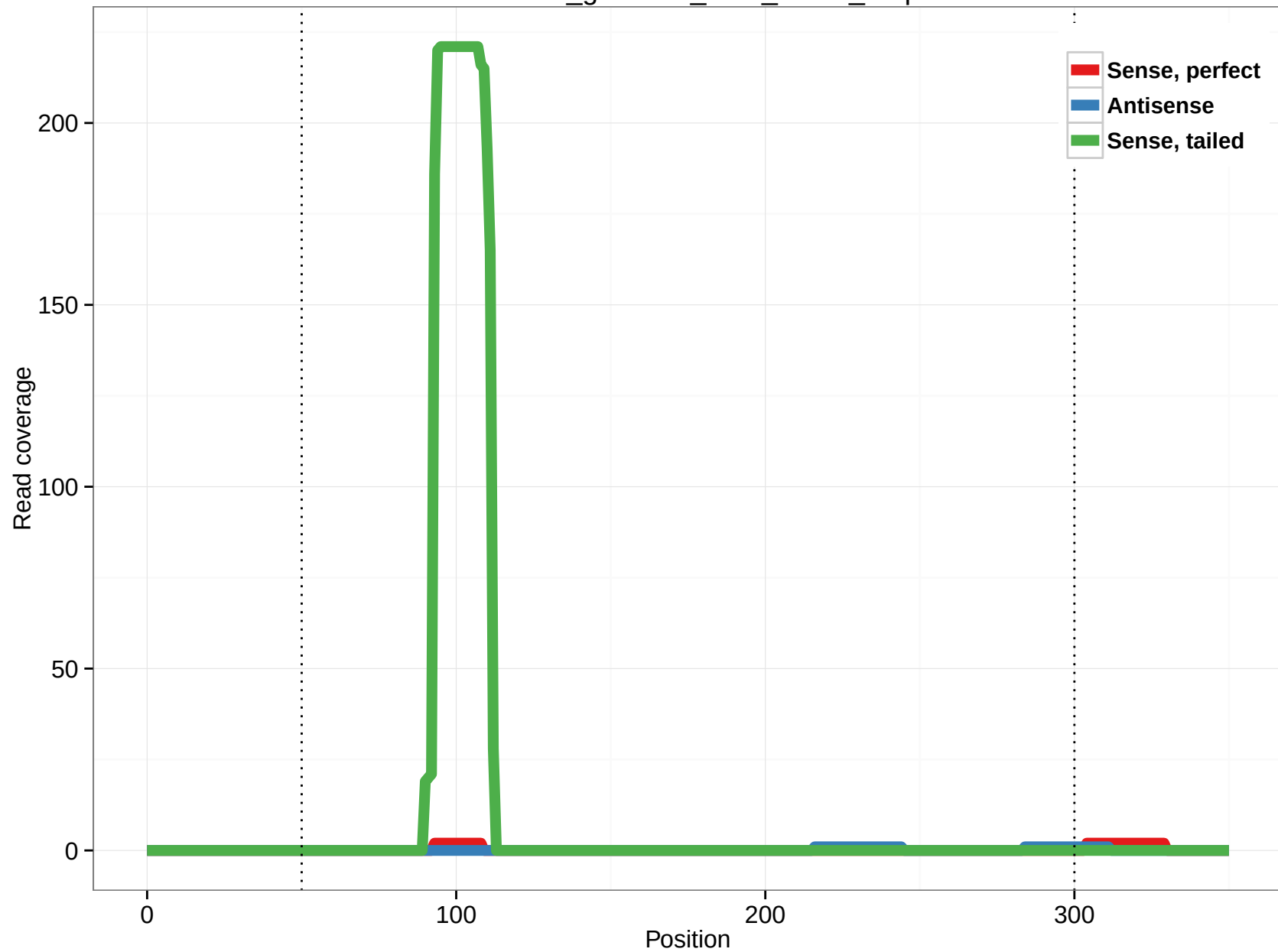
rheMac3_genscan_chr3_217.6_3.3p
