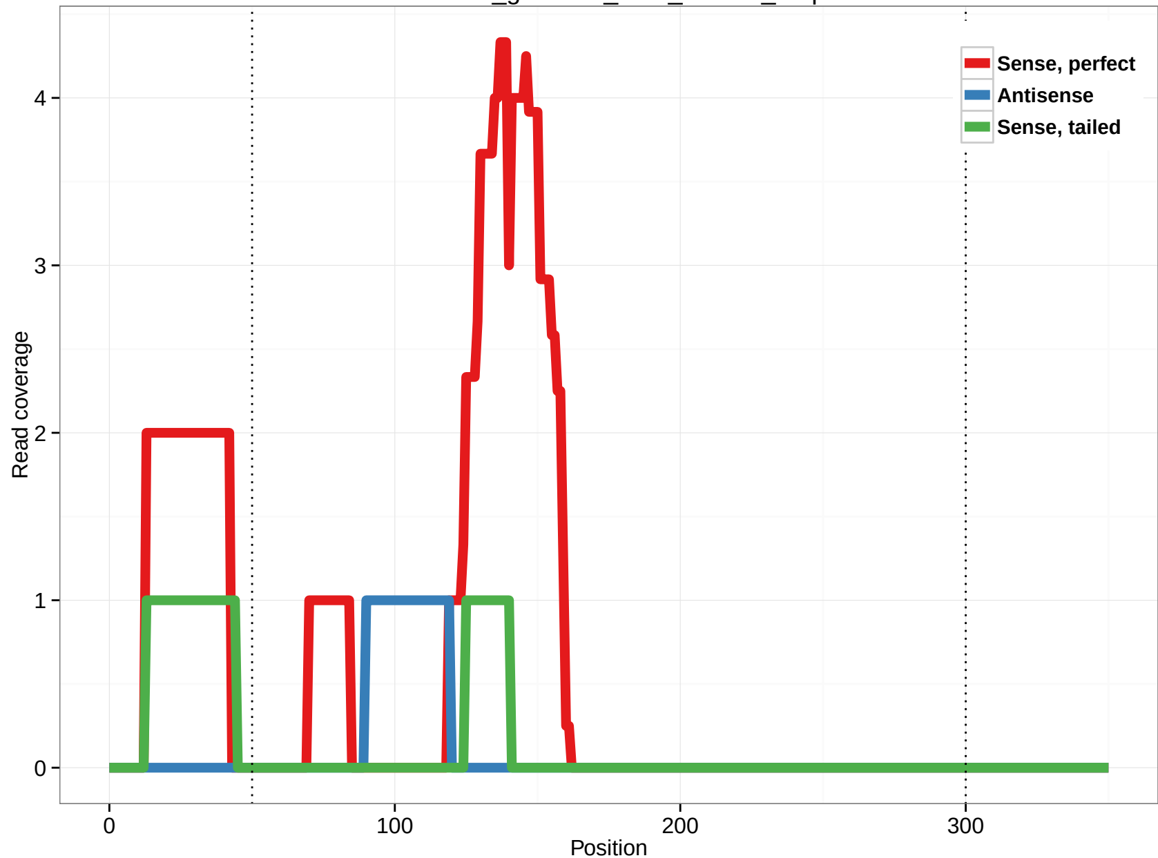
rheMac3_genscan_chr3_214.13_0.5p
