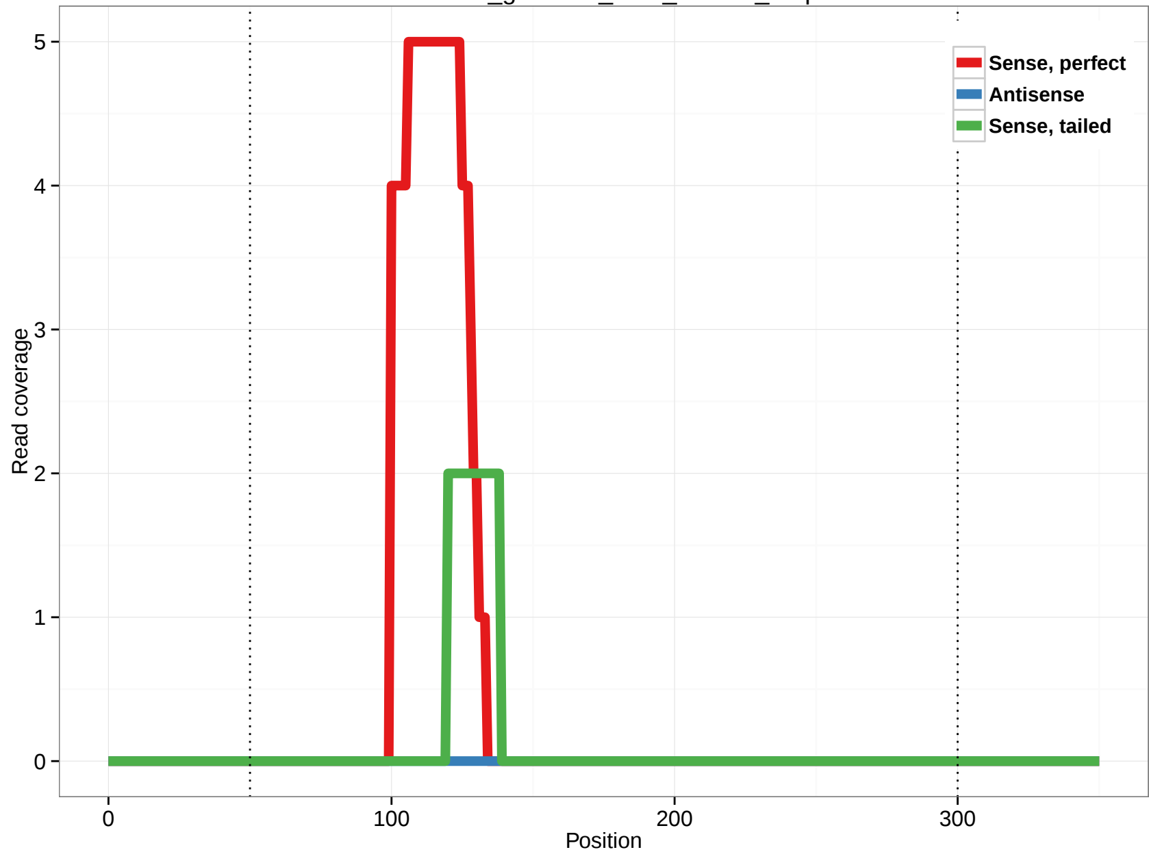
rheMac3_genscan_chr3_210.10_0.5p
