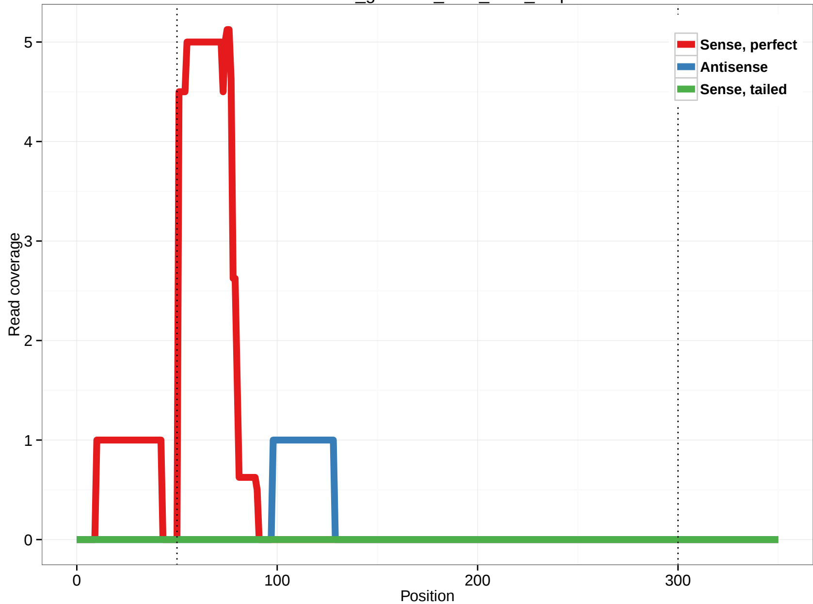
rheMac3_genscan_chr3_21.8_2.5p
