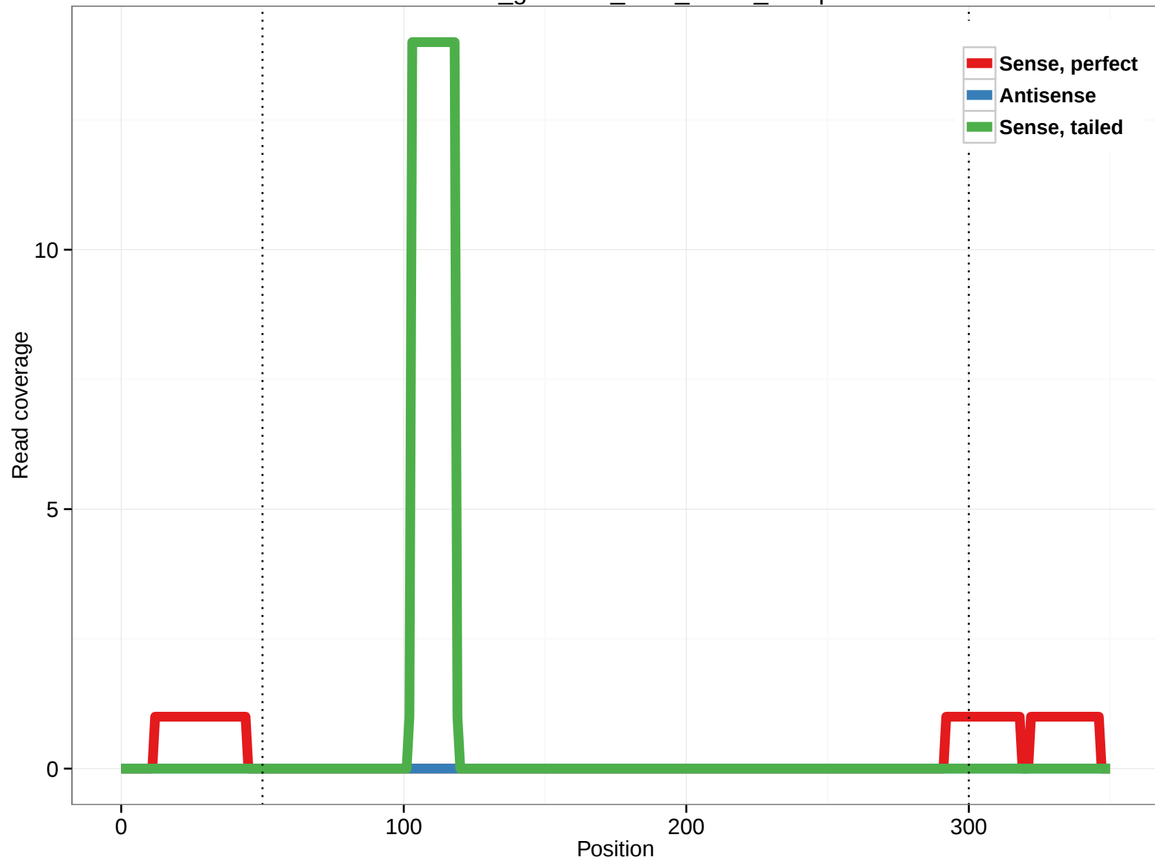
rheMac3_genscan_chr3_21.37_36.5p
