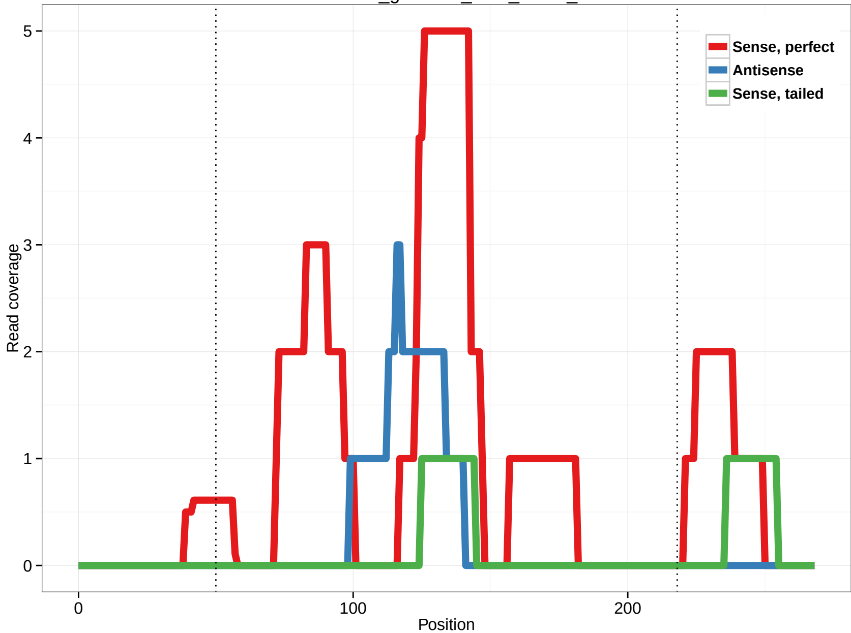
rheMac3_genscan_chr3_21.31_0
