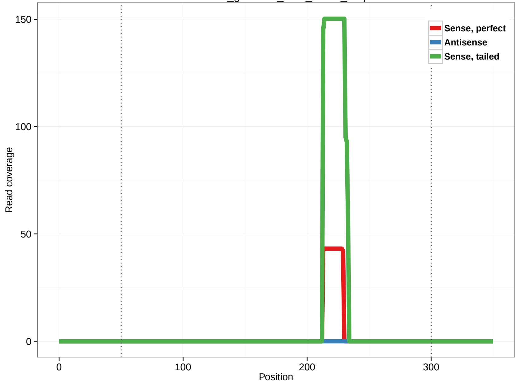
rheMac3_genscan_chr3_21.12_6.5p
