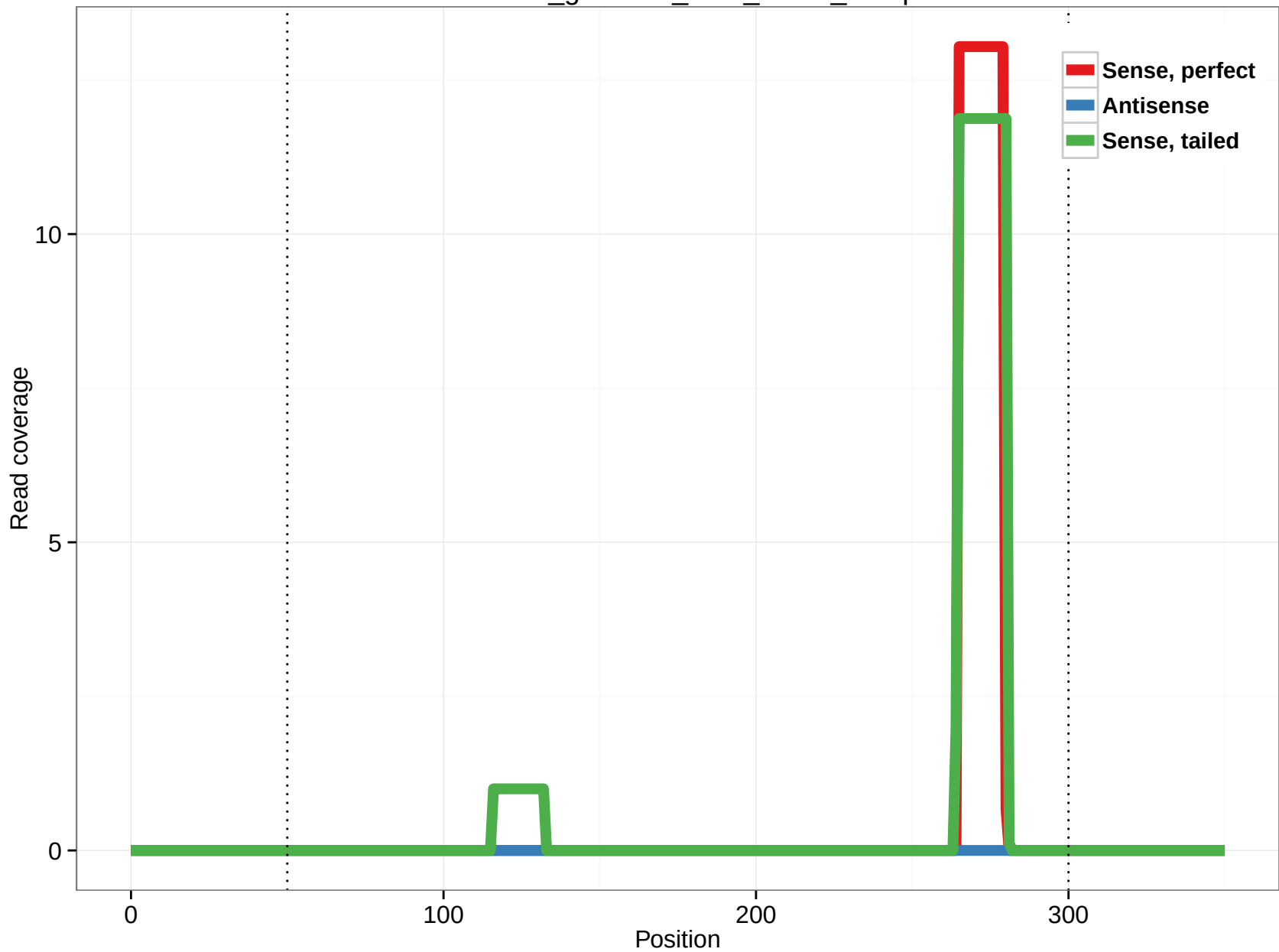
rheMac3_genscan_chr3_196.7_31.5p
