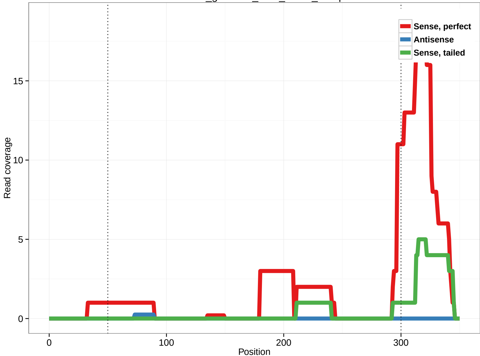
rheMac3_genscan_chr3_196.7_14.3p
