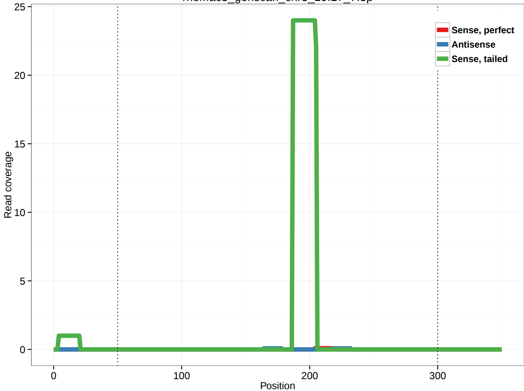
rheMac3_genscan_chr3_19.17_7.3p
