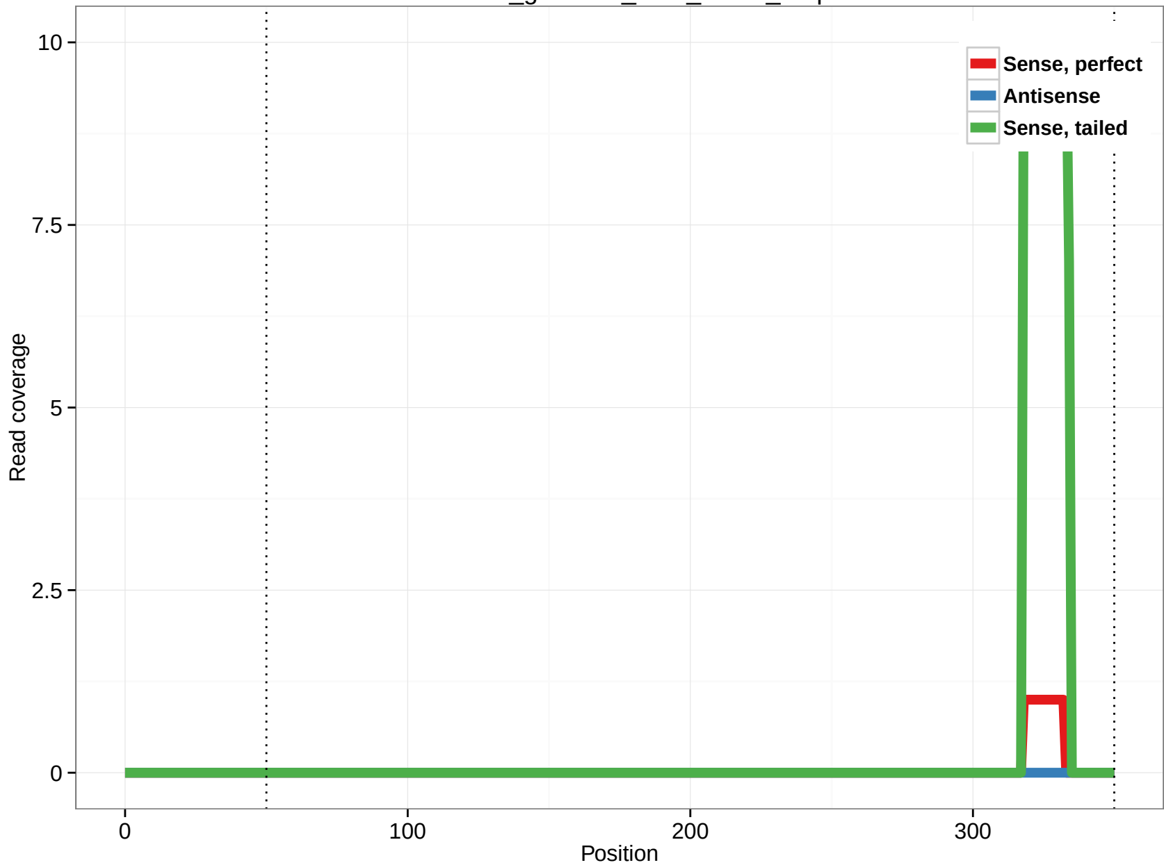
rheMac3_genscan_chr3_18.11_1.5p
