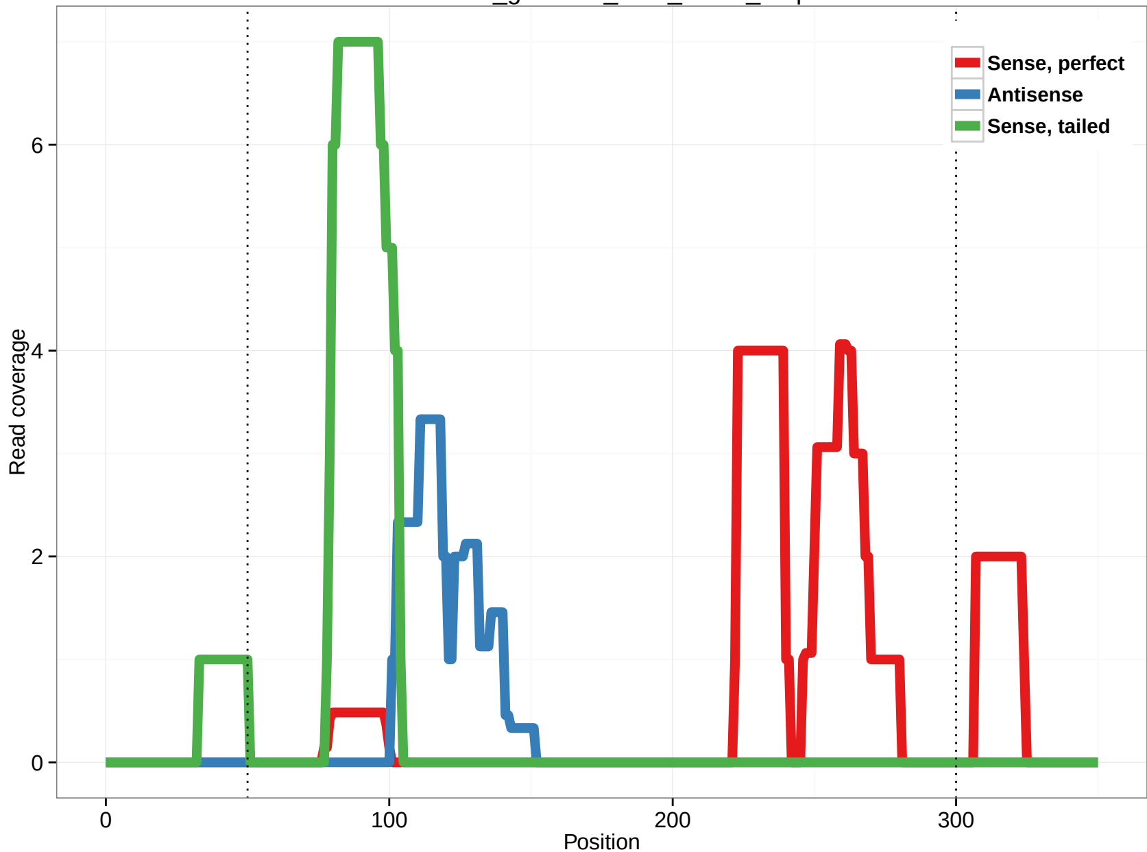
rheMac3_genscan_chr3_160.3_2.5p
