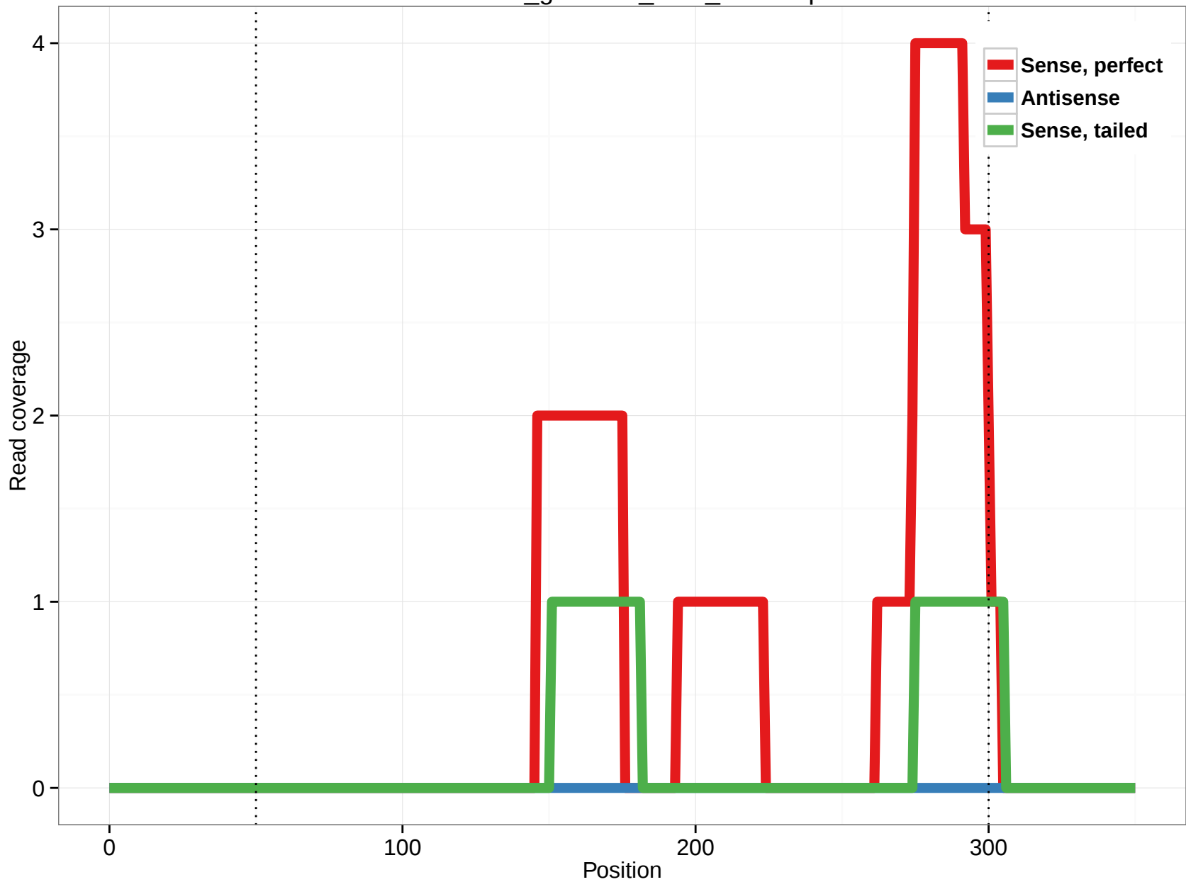
rheMac3_genscan_chr3_16.39.3p
