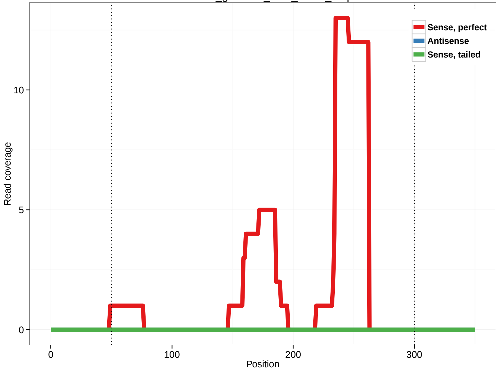
rheMac3_genscan_chr3_16.16_1.5p
