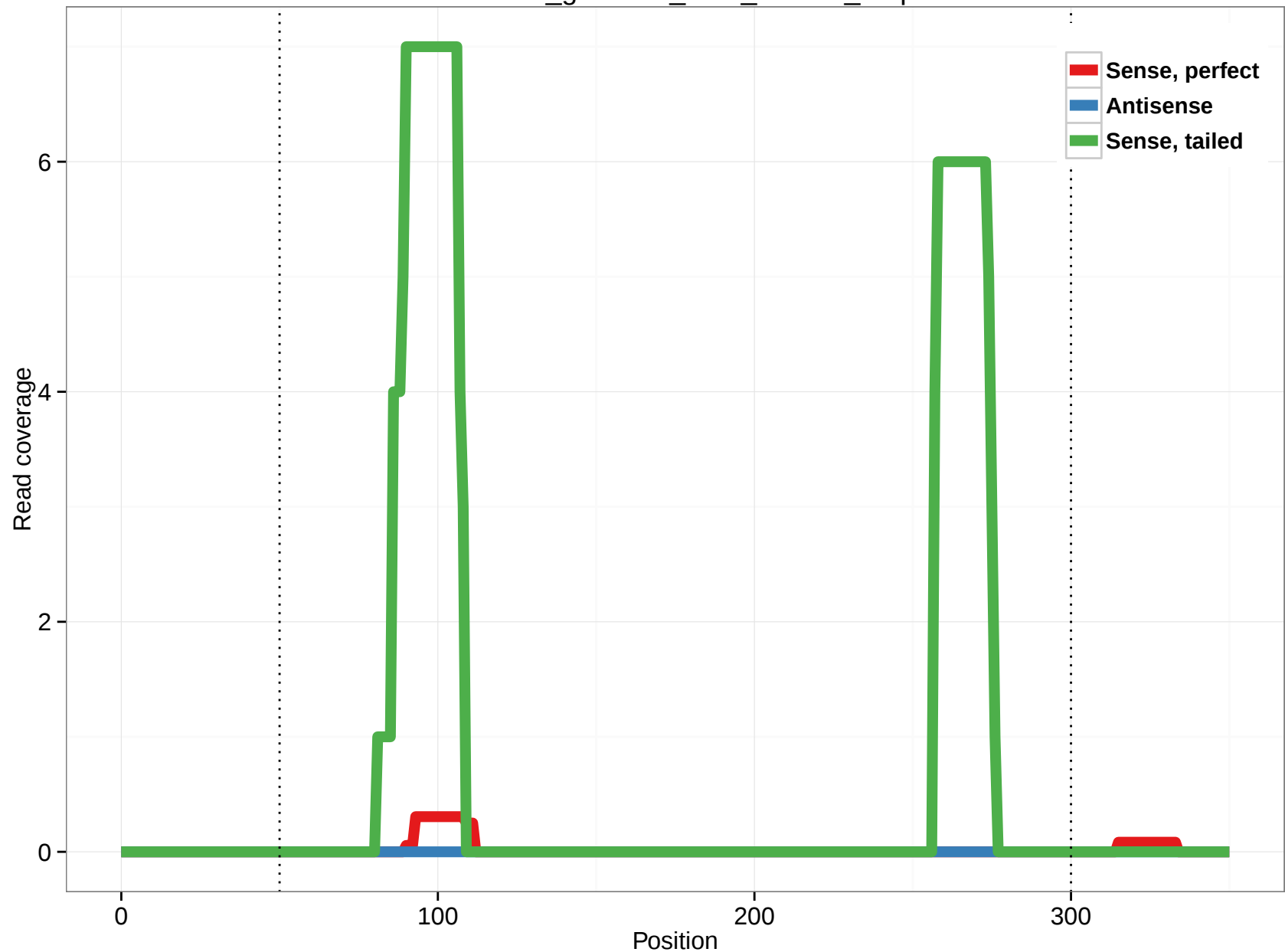
rheMac3_genscan_chr3_159.17_6.5p
