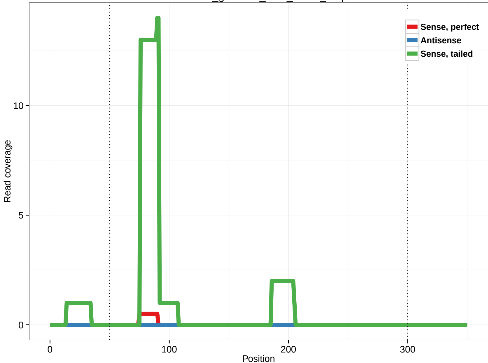
rheMac3_genscan_chr3_156.8_6.3p
