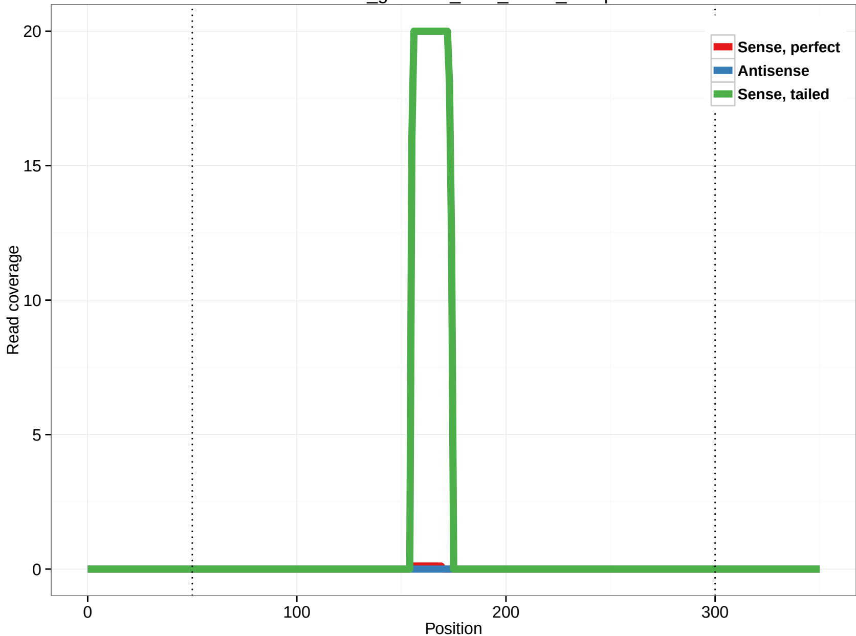
rheMac3_genscan_chr3_156.5_14.3p
