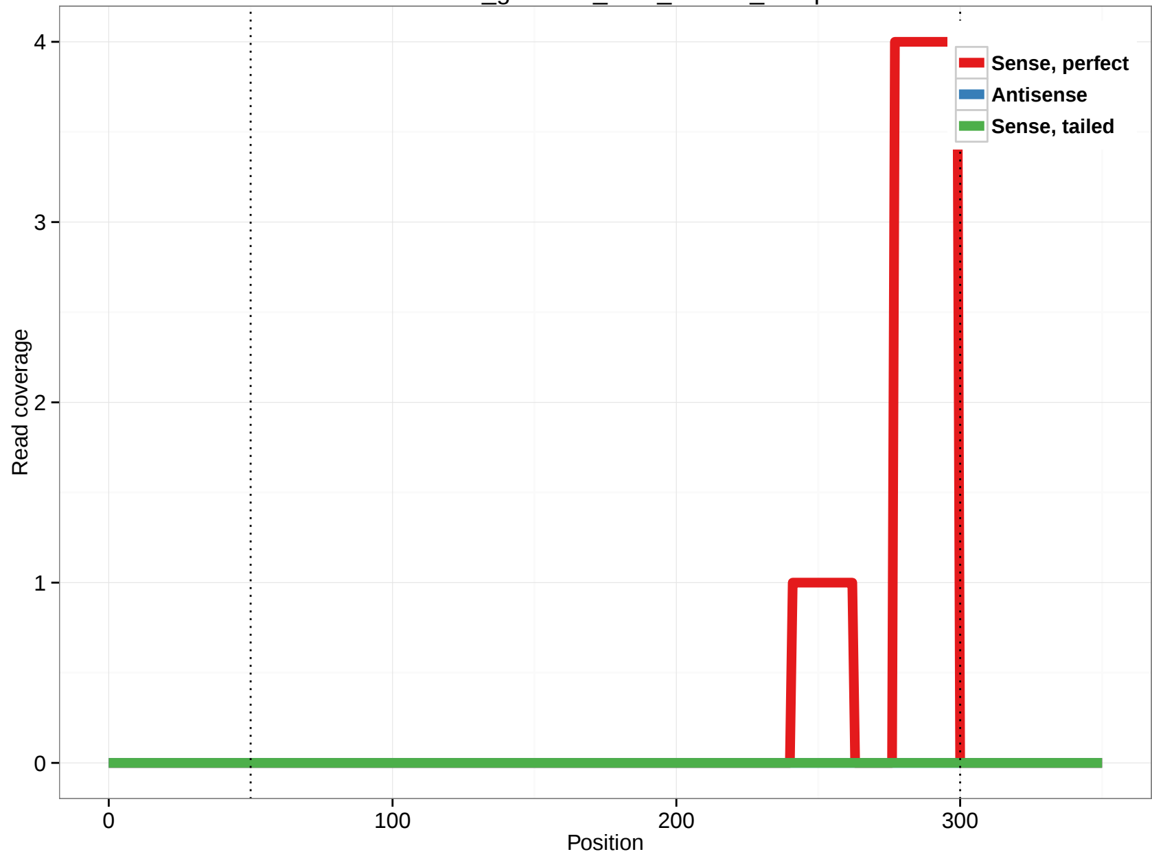
rheMac3_genscan_chr3_155.24_13.3p
