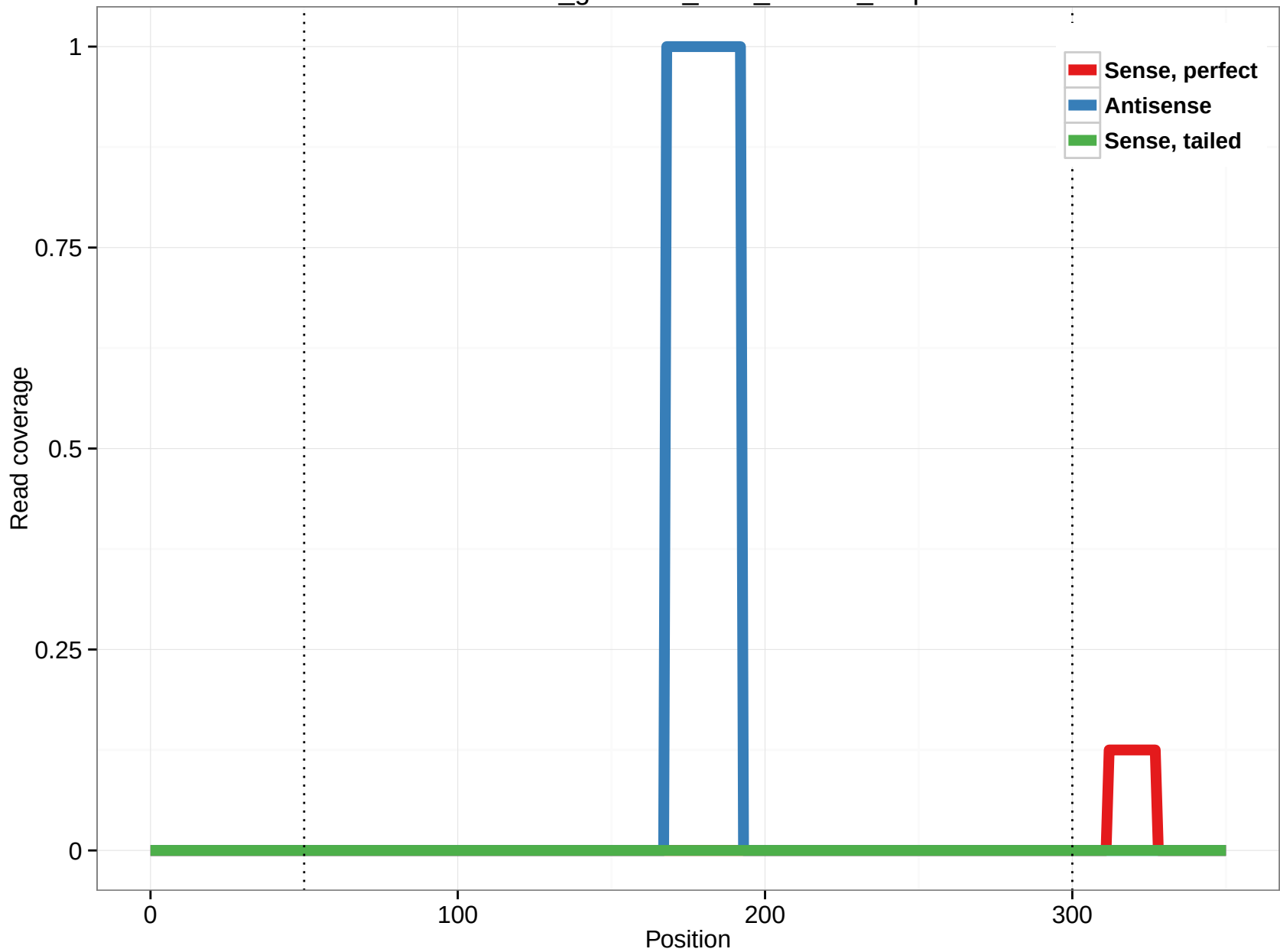
rheMac3_genscan_chr3_155.22_9.5p
