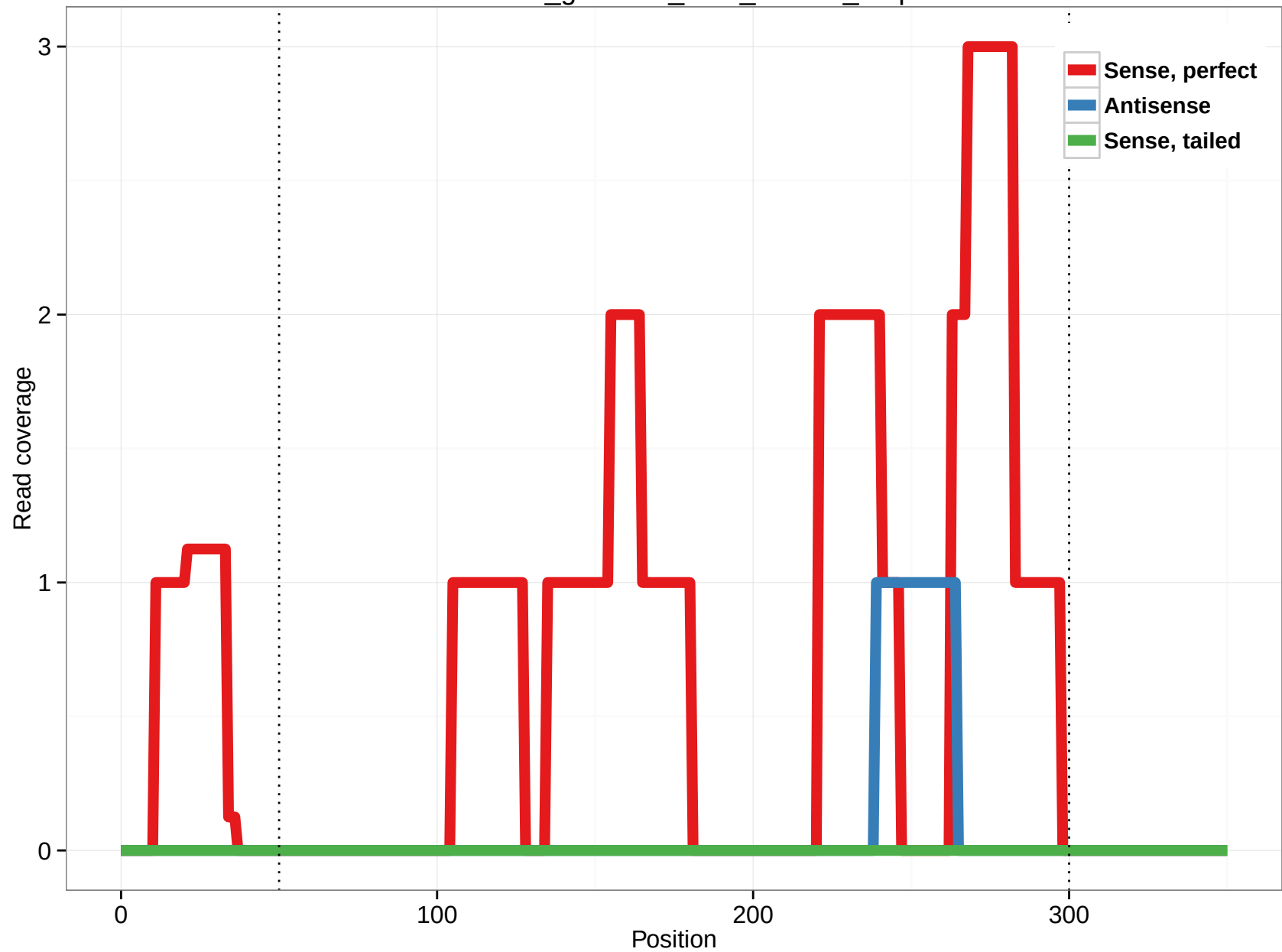
rheMac3_genscan_chr3_155.12_4.5p
