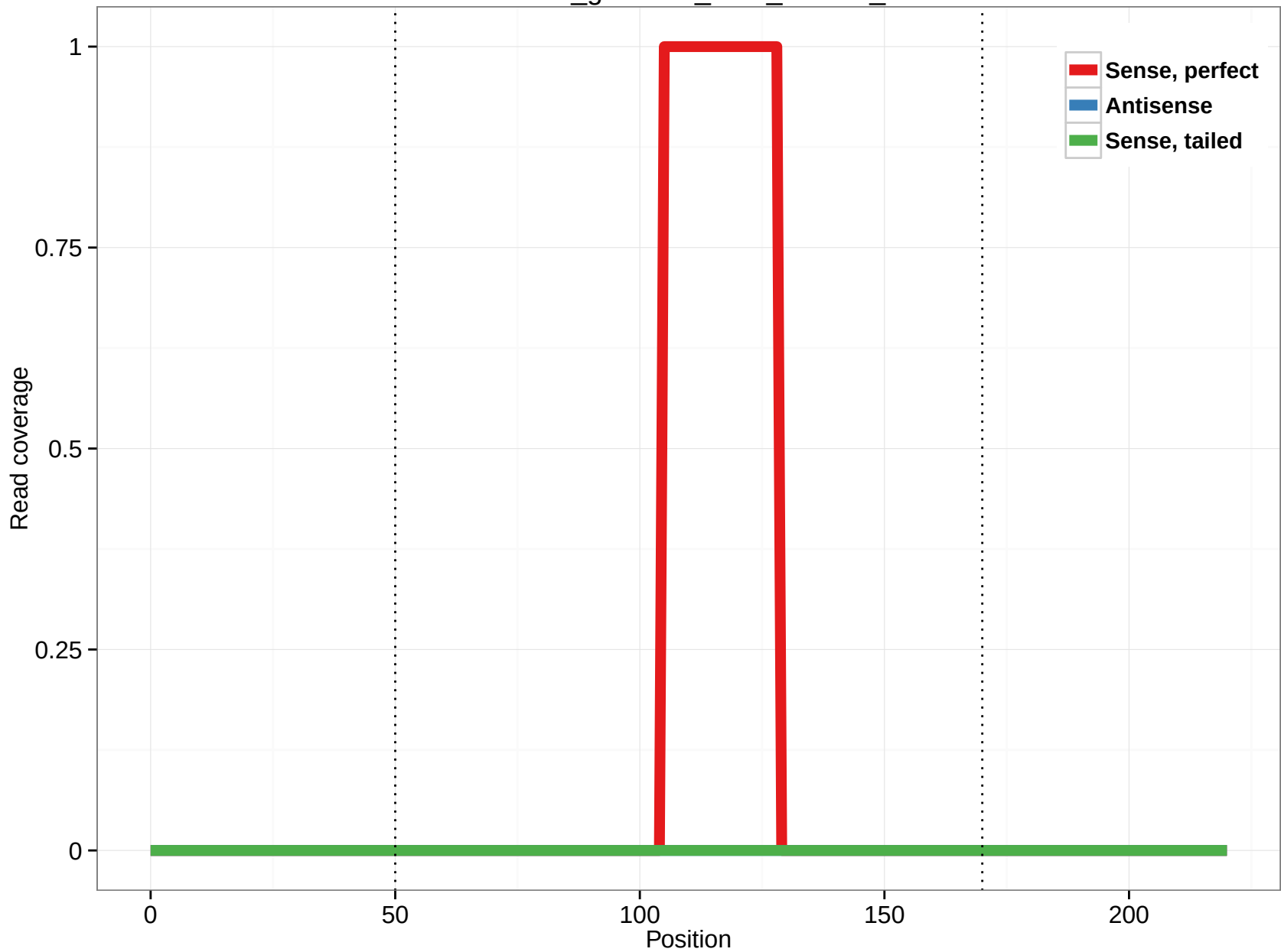
rheMac3_genscan_chr3_155.12_13
