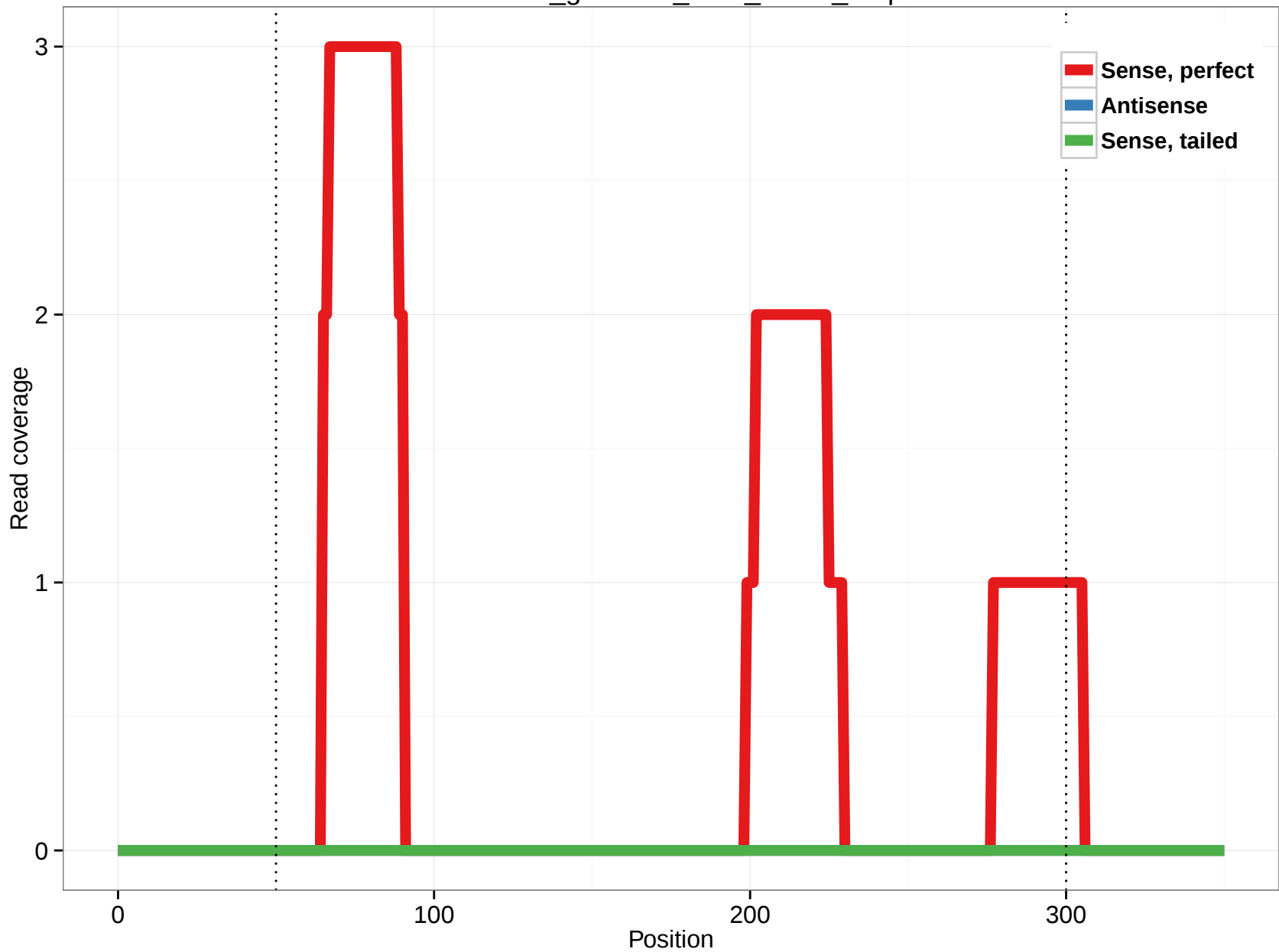
rheMac3_genscan_chr3_151.2_6.5p
