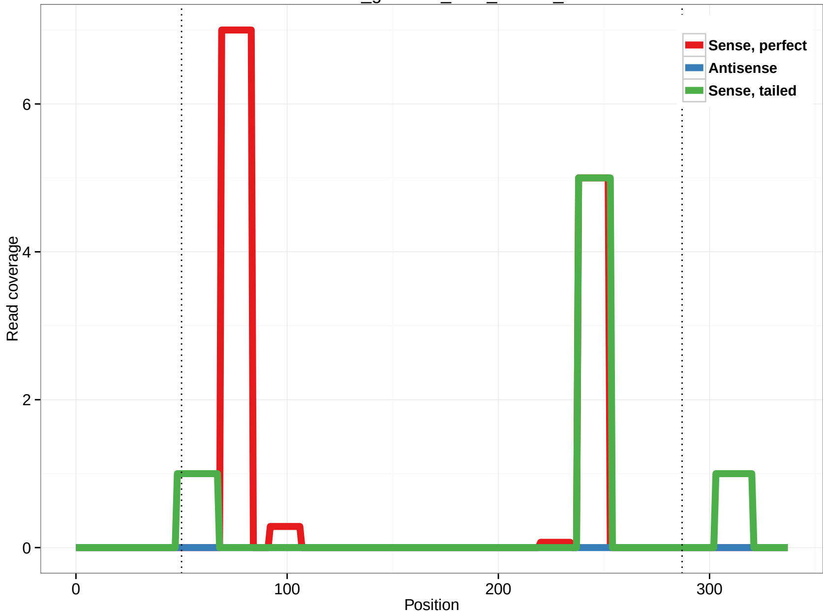
rheMac3_genscan_chr3_146.20_5
