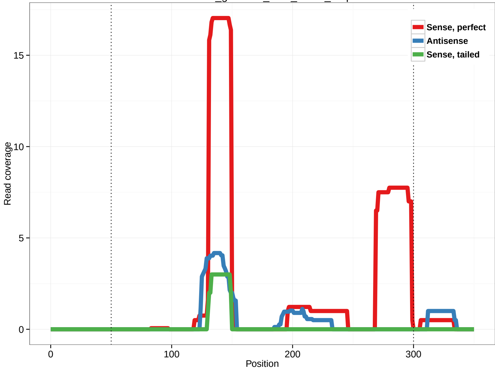
rheMac3_genscan_chr3_144.1_5.5p
