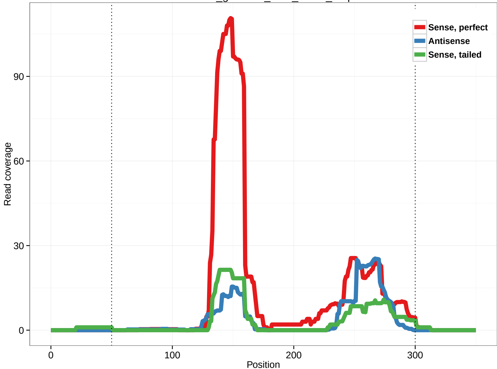
rheMac3_genscan_chr3_144.1_0.5p
