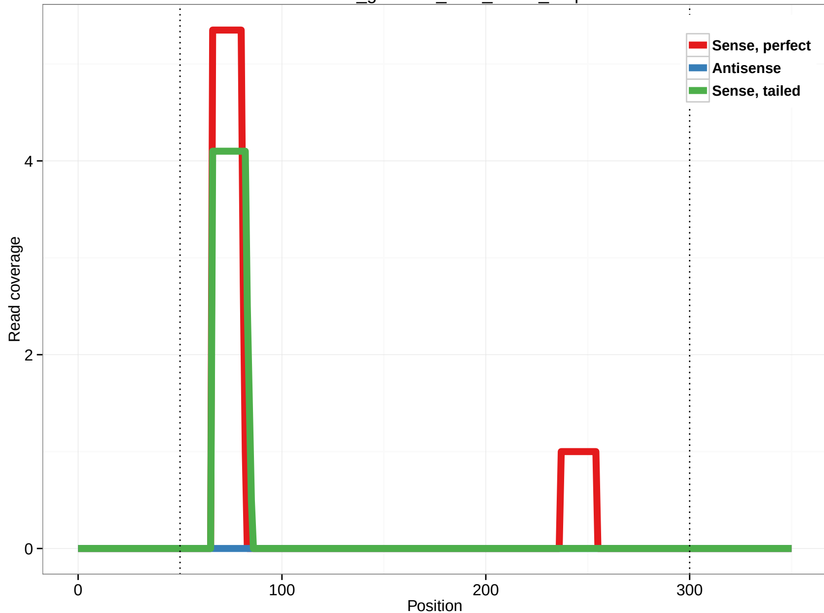
rheMac3_genscan_chr3_106.4_4.3p
